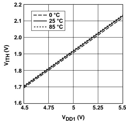
Figure 2. Typical Input Voltage Switching Threshold vs. Input Supply
