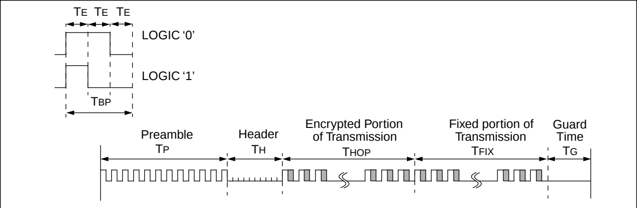
FIGURE 8-3: PREAMBLE/HEADER FORMAT
