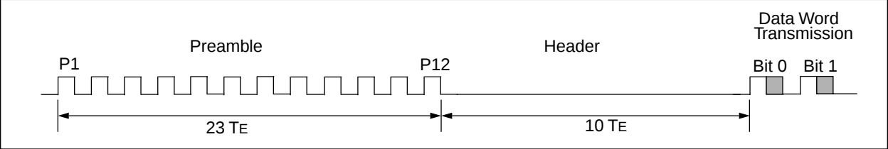
FIGURE 8-3: PREAMBLE/HEADER FORMAT
