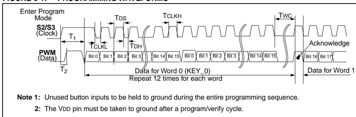
FIGURE 6-1: PROGRAMMING WAVEFORMS
