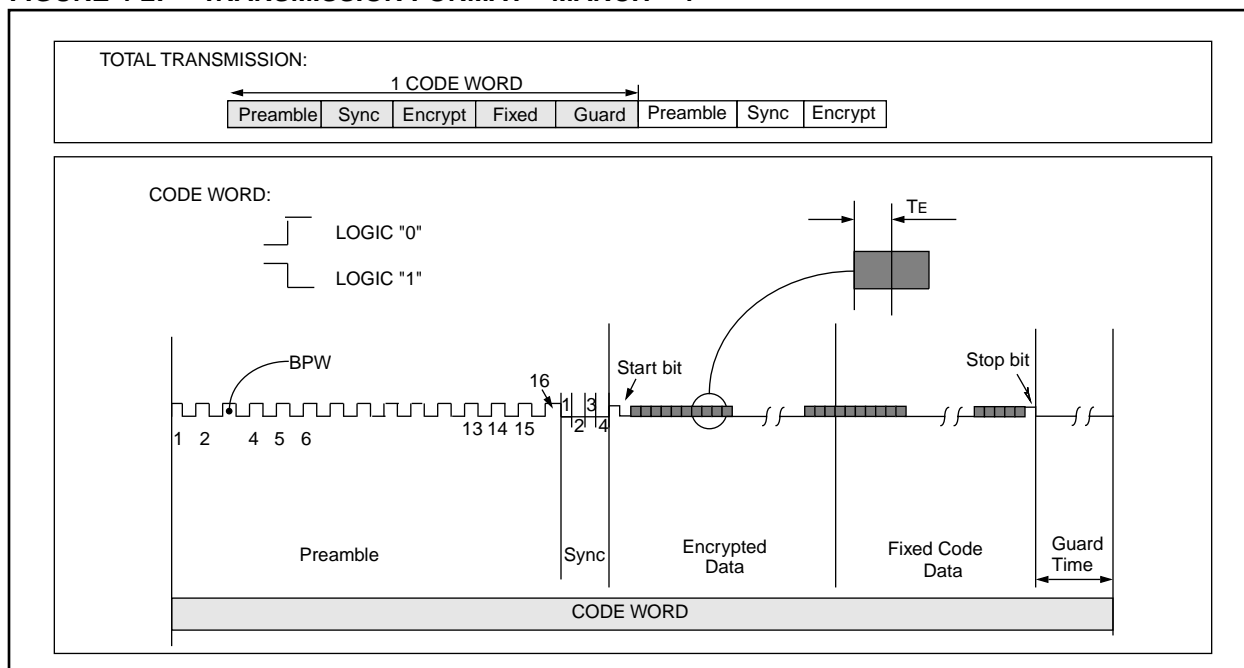
FIGURE 4-2: TRANSMISSION FORMAT—MANCH = 1
