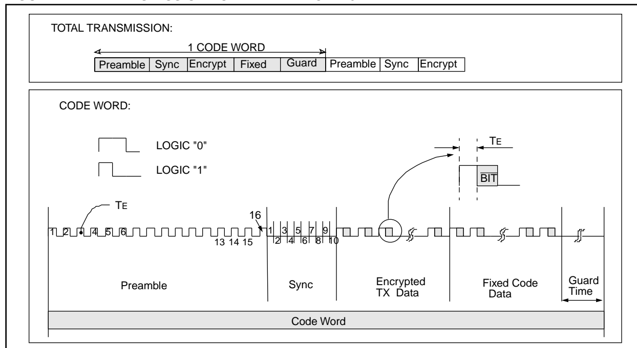
FIGURE 4-1: TRANSMISSION FORMAT—MANCH = 0
