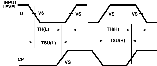
FIGURE 2. DATA SET-UP AND HOLD TIMES
