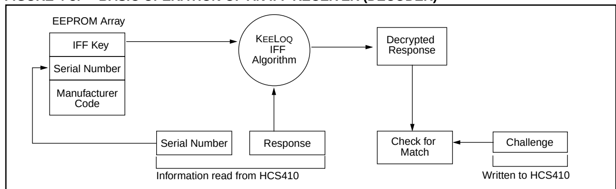
FIGURE 4-8: BASIC OPERATION OF AN IFF RECEIVER (DECODER)
