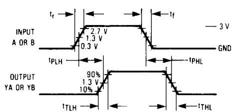
Figure 1. Switching Waveforms
