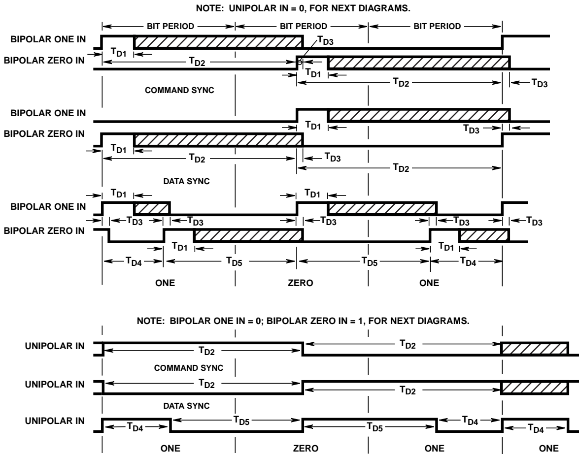
FIGURE 12. DECODER TIMING
