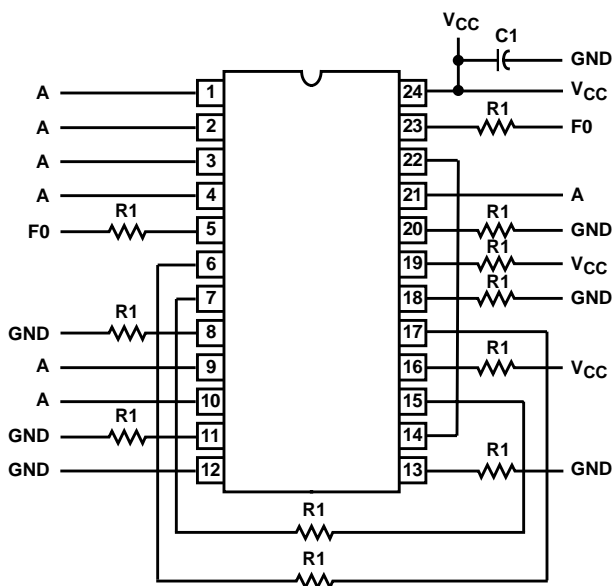
HD1-15530 Cerdip
