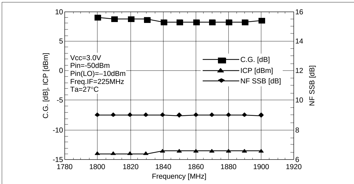
Figure 12 Gain, NF, ICP vs. Frequency
