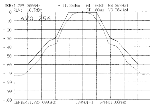
c-1. Spectrum1(1785MHz,PN9)
