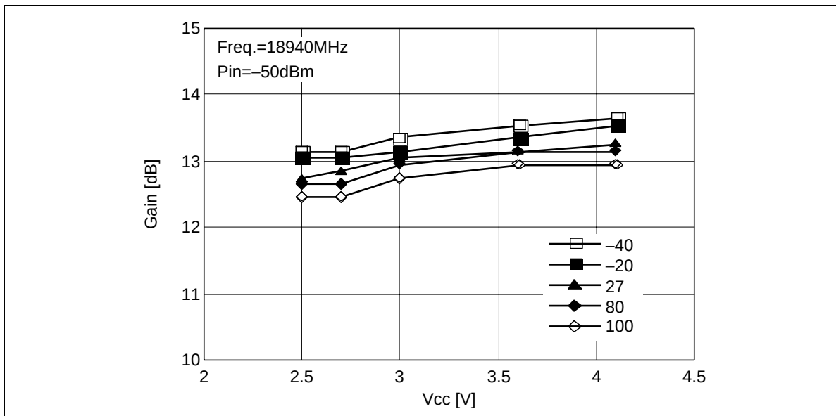
Figure 7 Gain vs. Supply Voltage
