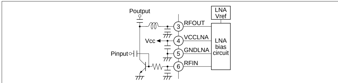
Figure 1 LNA Bias Circuit
