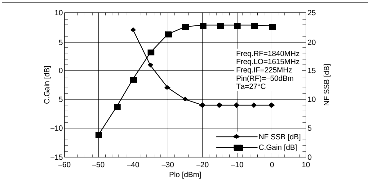
Figure 14 CG, NF vs. Local Input Power
