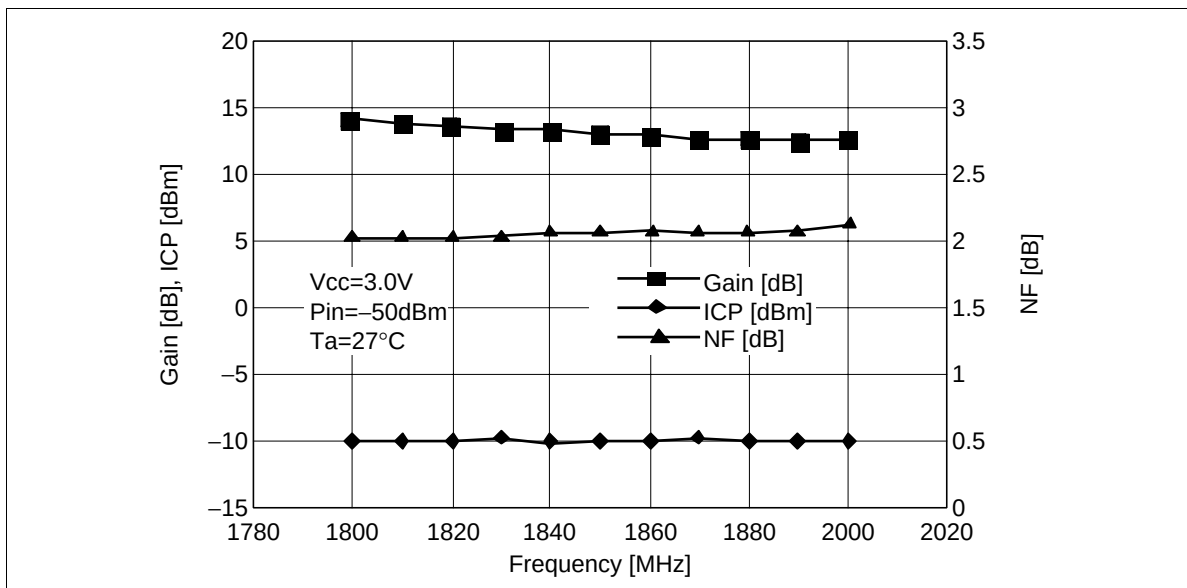
Figure 5 Gain, NF, ICP vs. Frequency
