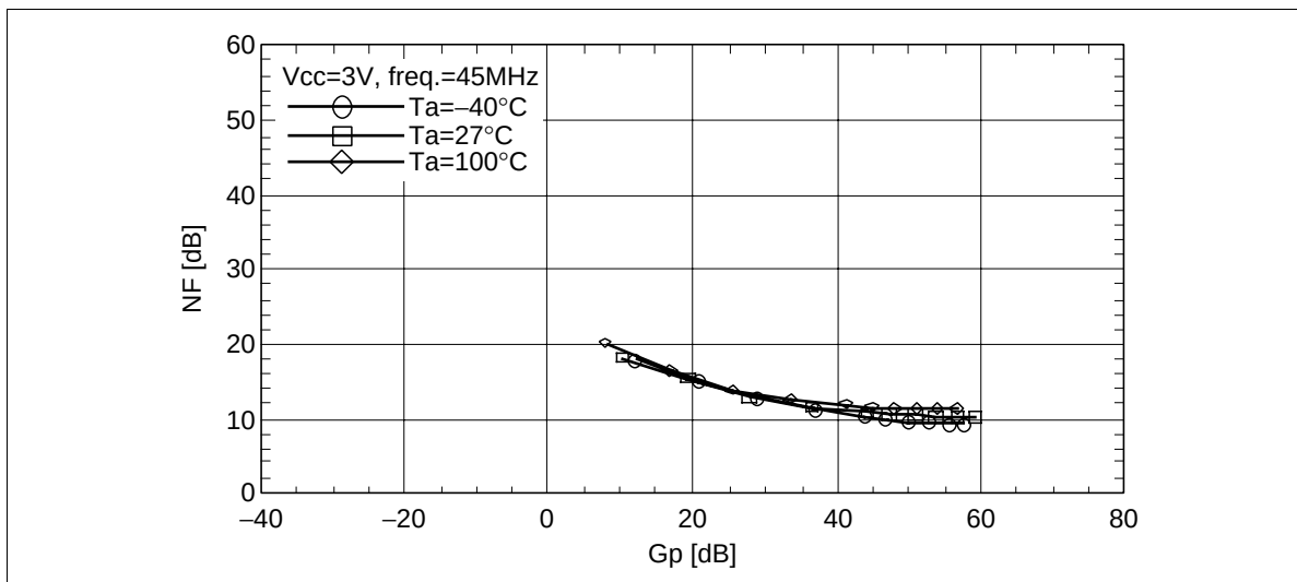
Figure 28 Noise Figure(NF) vs. Power Gain(Gp)
