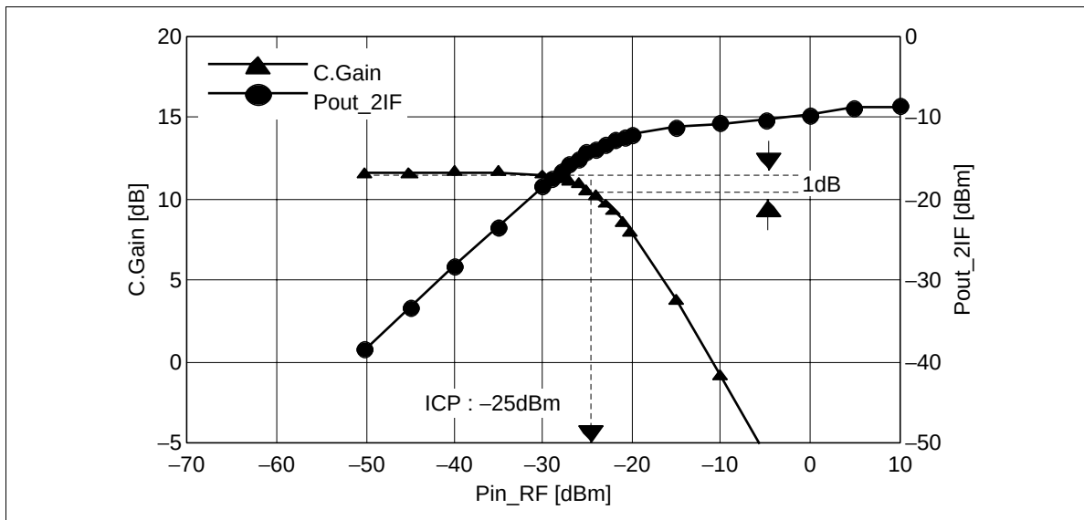
Figure 20 Input-Output Characteristics, 1dB-Compression Point
