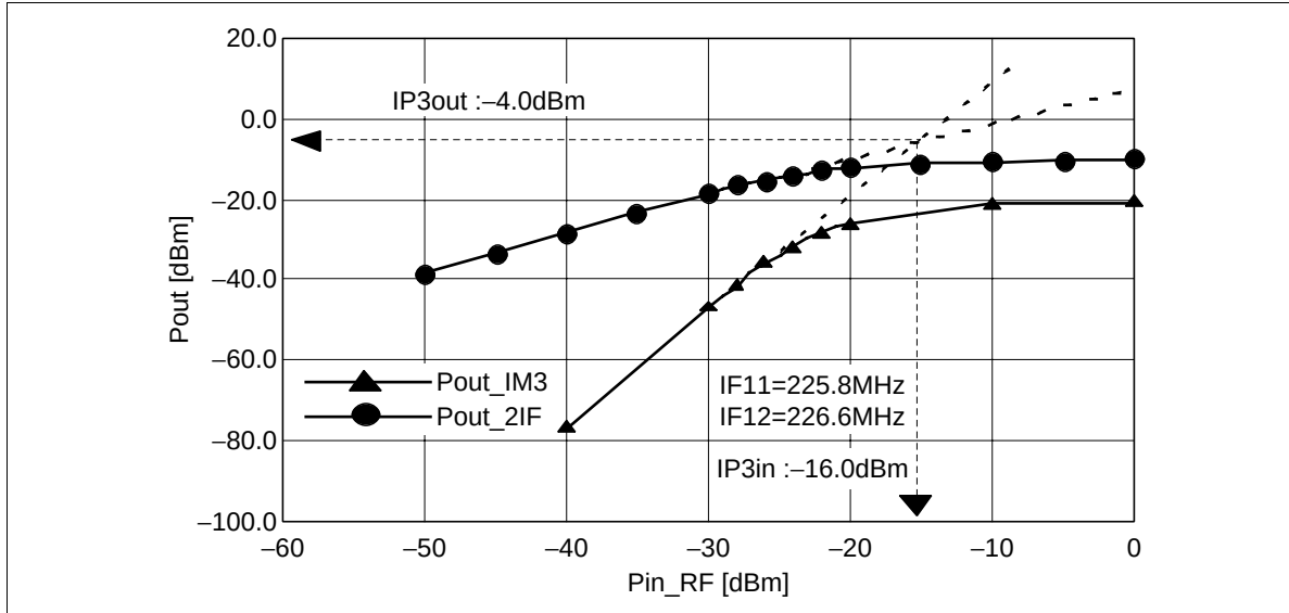
Figure 21 Intermodulation 3rd Characteristics
