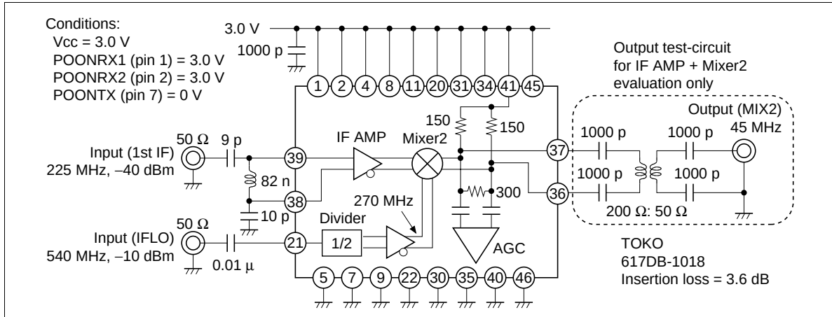
Figure 19 Evaluation Circuit for IF AMP + 2nd Mixer
