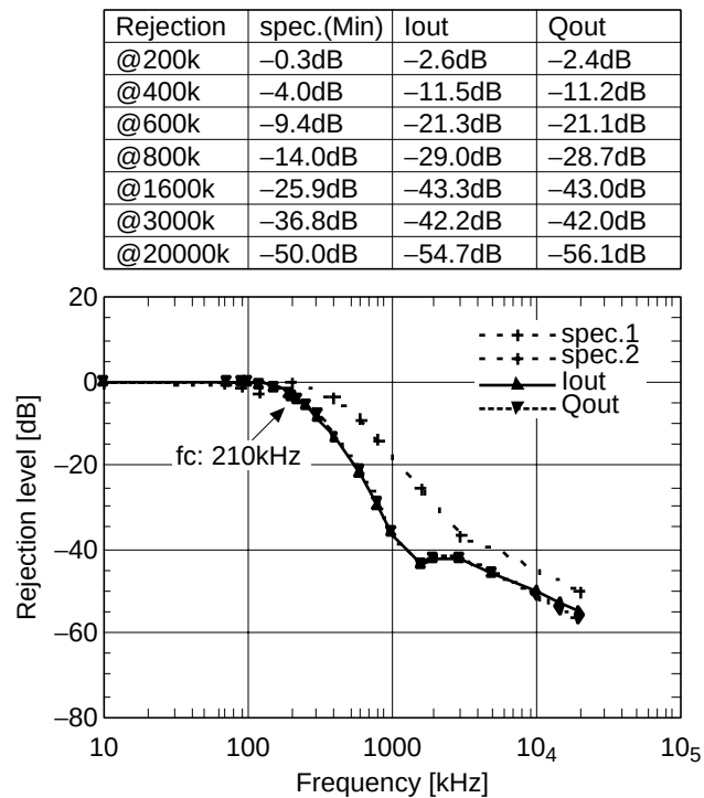
Figure 35 Internal LPF Frequency Characteristics
