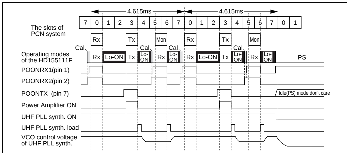
Figure 2 Control Diagram for Operating Mode Selection
