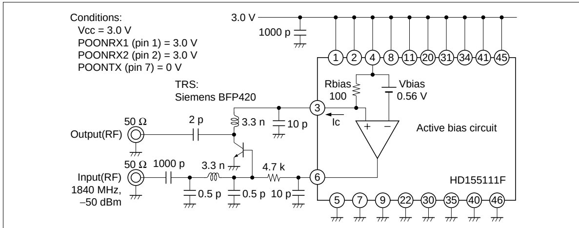
Figure 4 Evaluation Circuit for LNA
