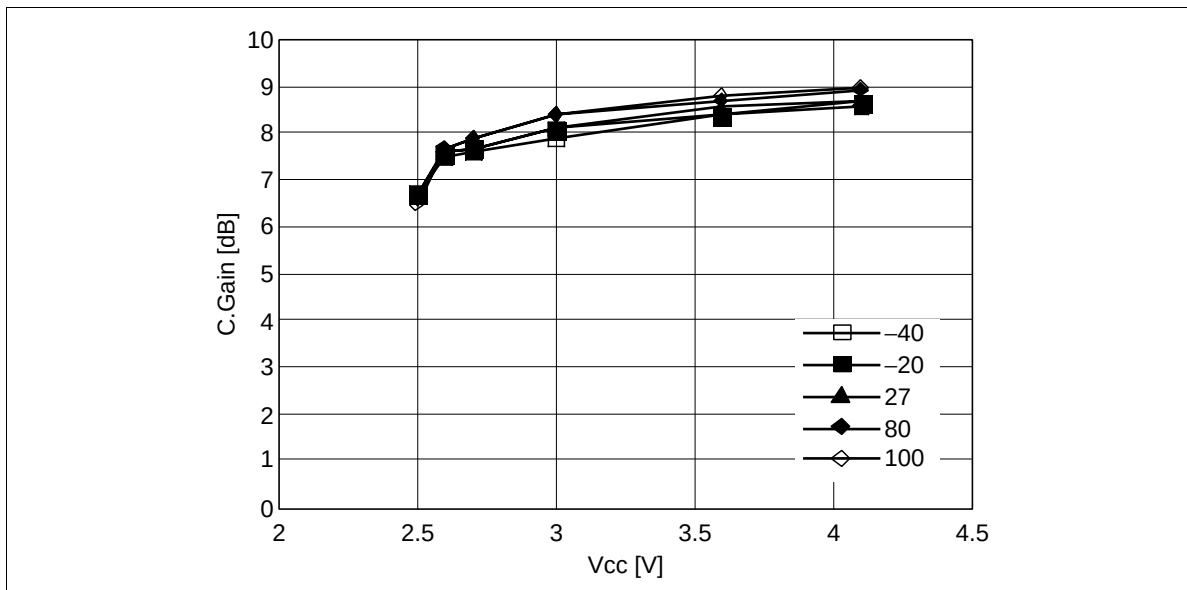
Figure 16 Gain vs. Supply Voltage
