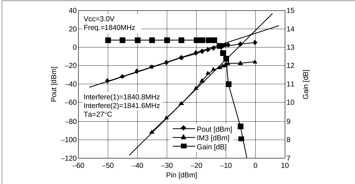
Figure 6 Gain, Pout vs. Pin
