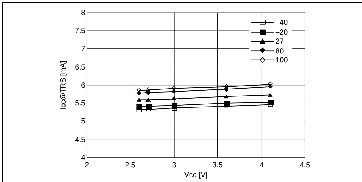
Figure 10 LNA Transistor Current vs. Supply Voltage
