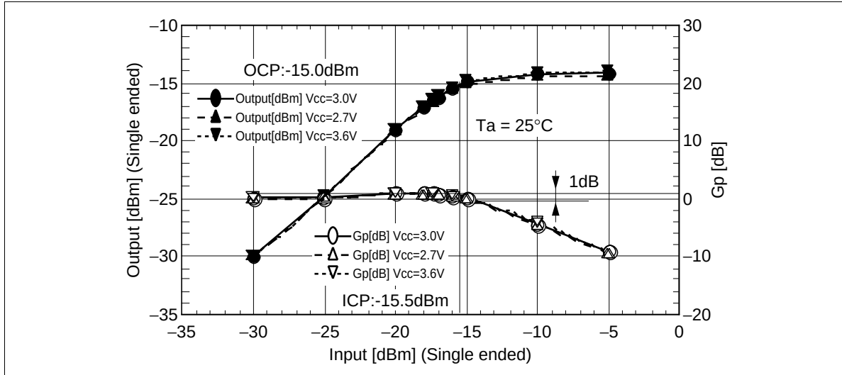
Figure 32 Input-Output Characteristics
