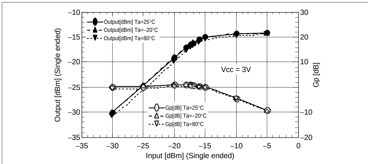
Figure 33 Input-Output Characteristics
