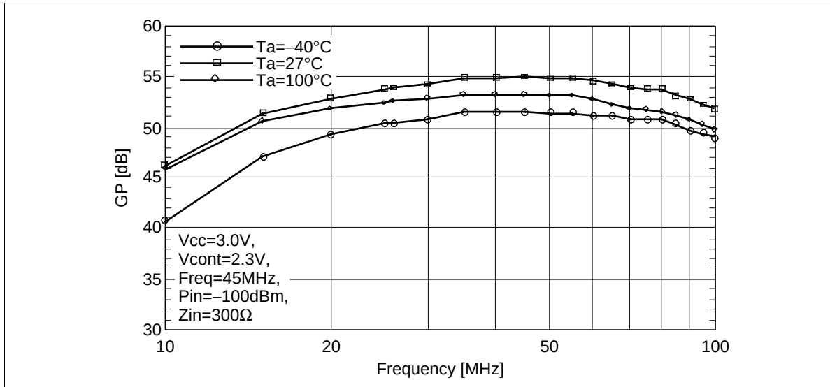
Figure 27 Power Gain vs. Frequency
