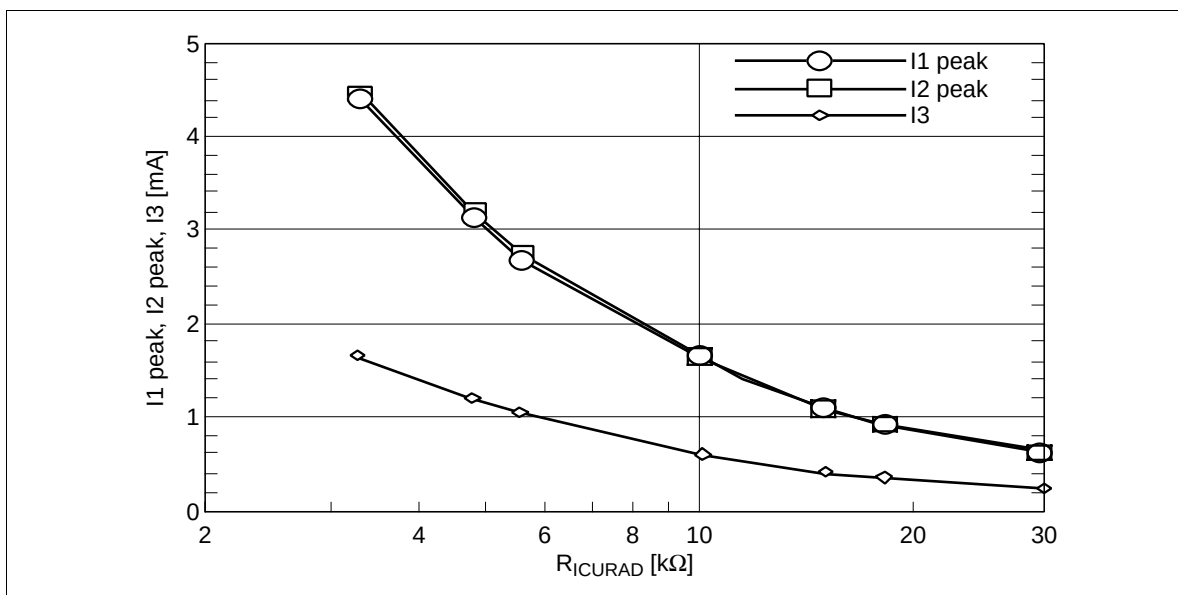
Figure 38 I1 Peak, I2 Peak, I3 vs. R ICURAD Characteristics
