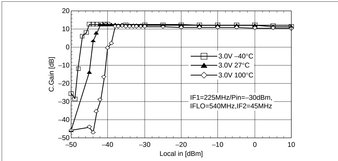
Figure 22 C.Gain vs. Local in Power
