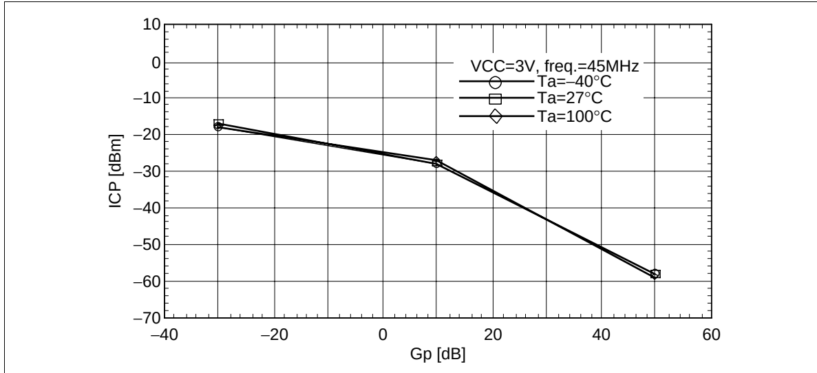
Figure 29 Input Compression Point(ICP) vs. Power Gain(Gp)
