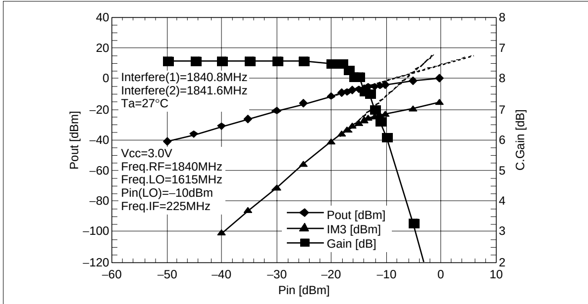
Figure 13 Gain, Pout vs. Pin
