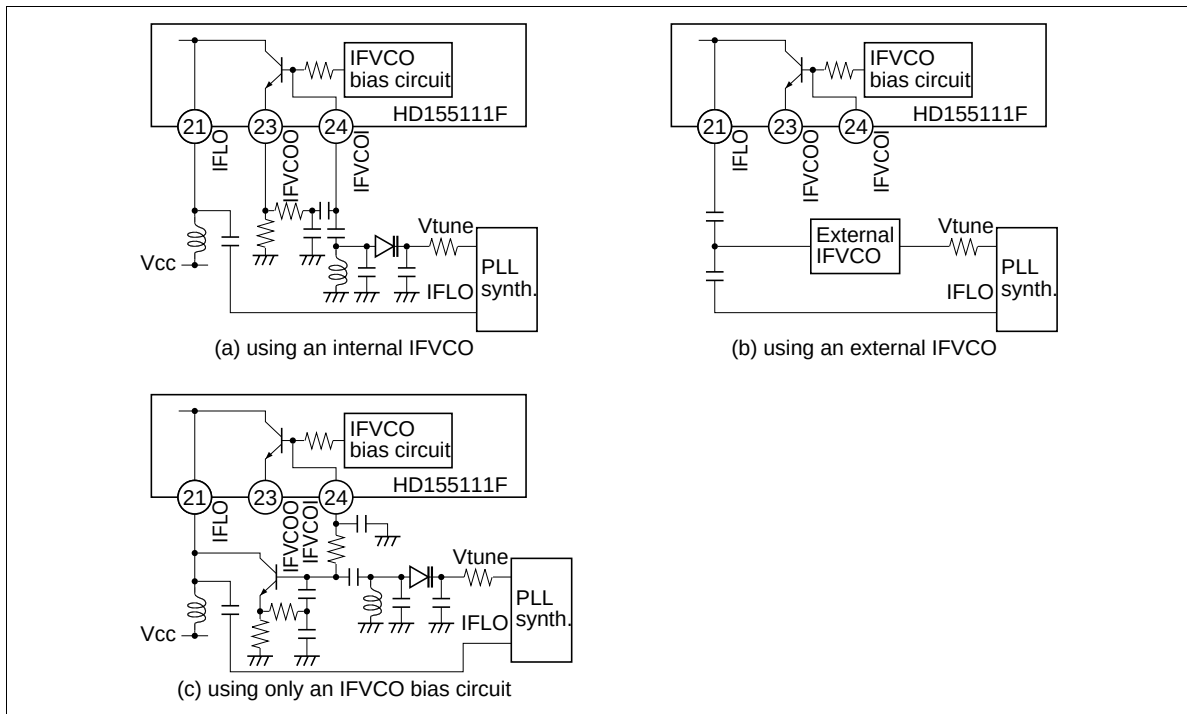
Figure 3 IFVCO Circuits
