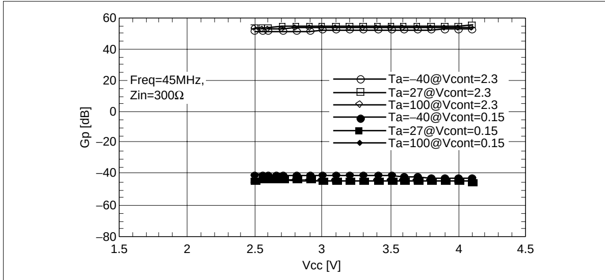
Figure 30 Power Gain(Gp) vs. Supply Voltage(Vcc)
