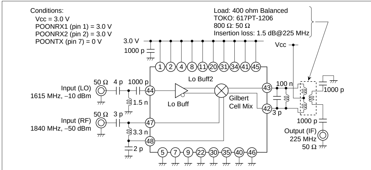
Figure 11 Evaluation Circuit for 1st Mixer
