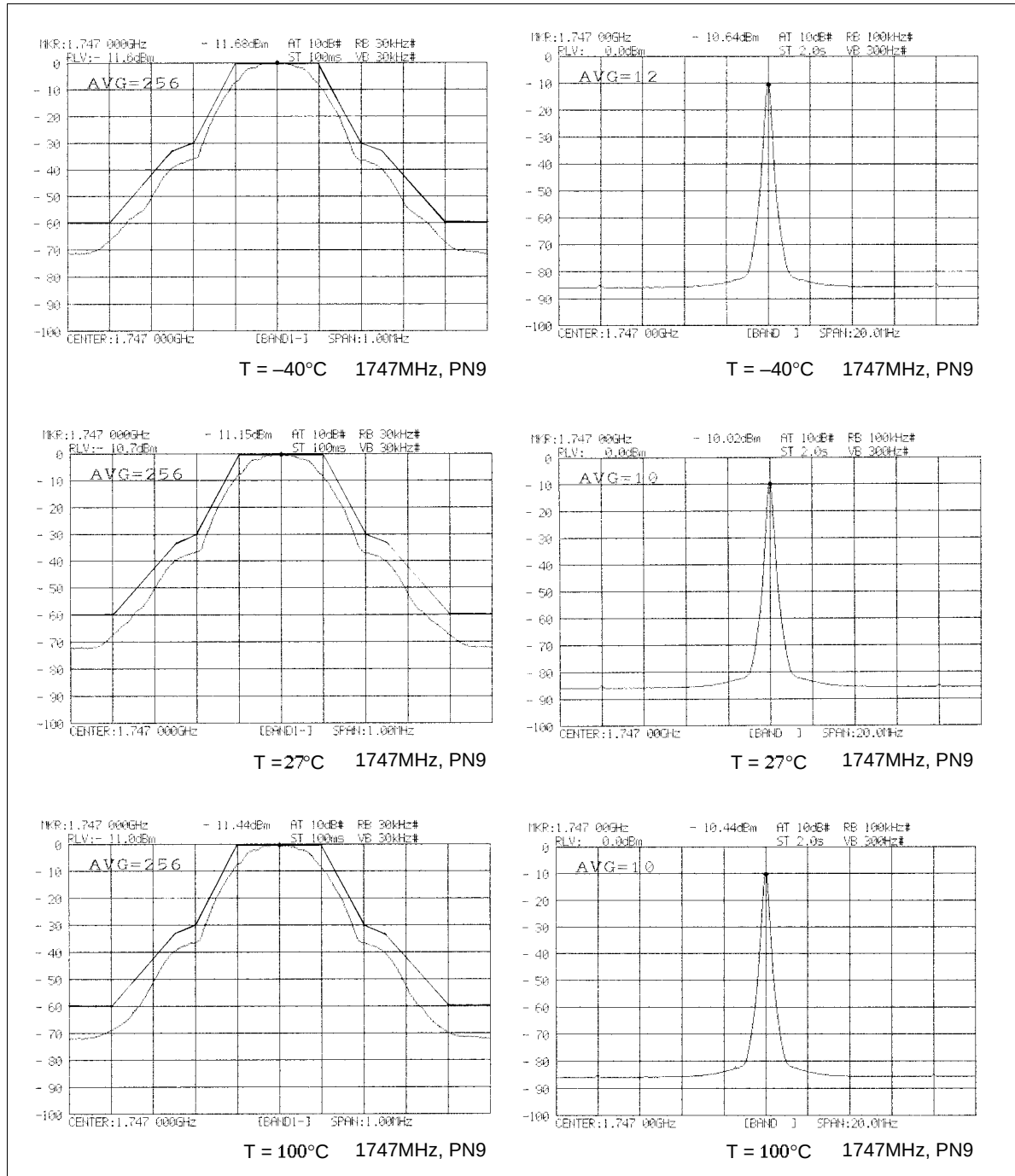
Figure 41 GMSK Modulated Transmitter Output Spectrum vs. Temperature
