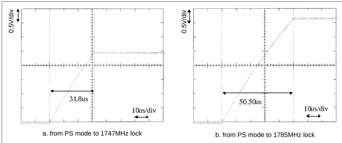
Figure 42 Acquisition Time (Lock Up Time)
