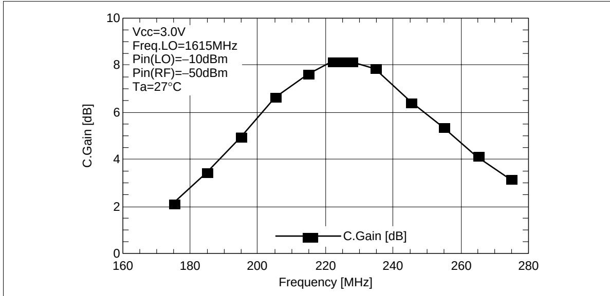
Figure 15 Output Frequency Characteristics
