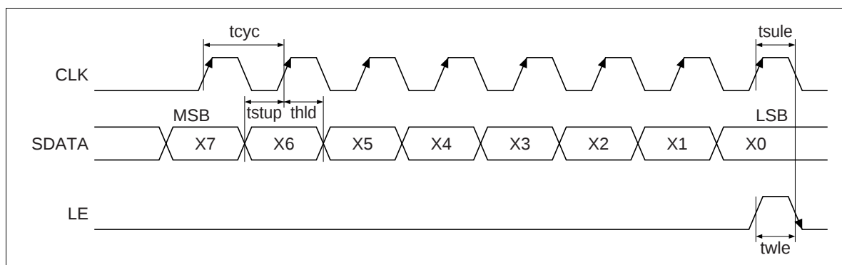
Figure 2 Three-Wire Bus Timing Diagram
