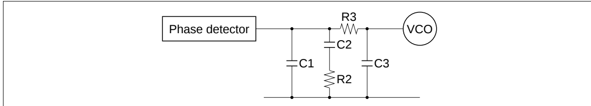
Figure A-1 Loop Filter Circuit of OPLL
