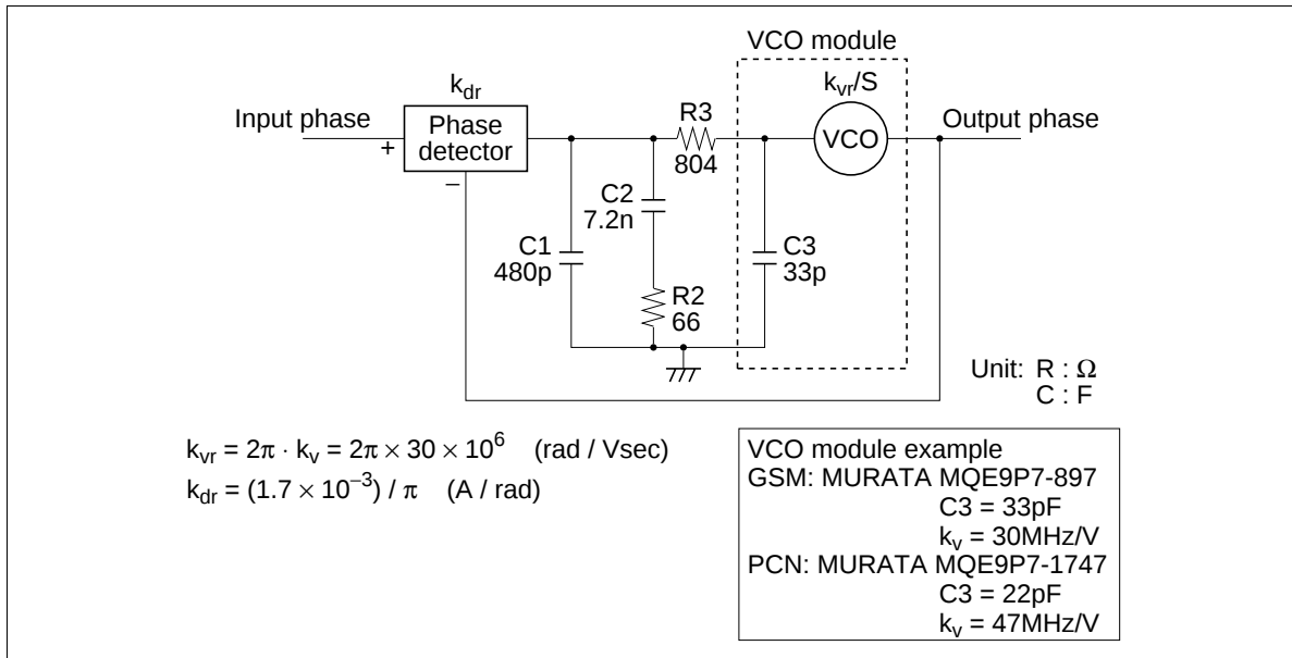
Figure A-2 Block Diagram for OPLL Simulation
