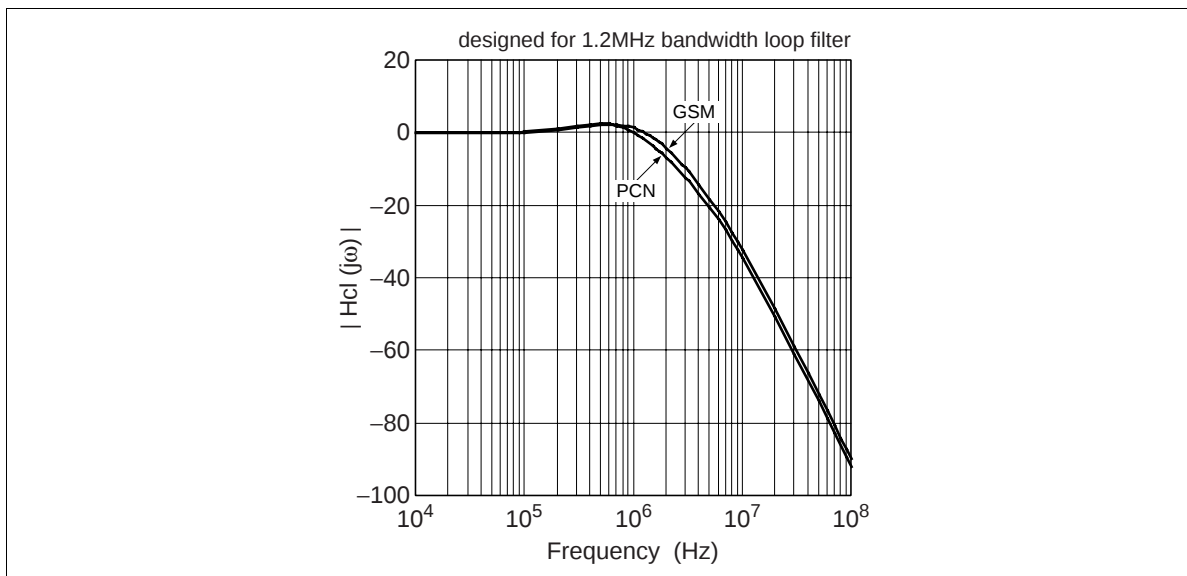
Figure A-4 The Magnitude, |Hcl(j\omega)| of Closed Loop Transfer Function Hcl(j\omega)
