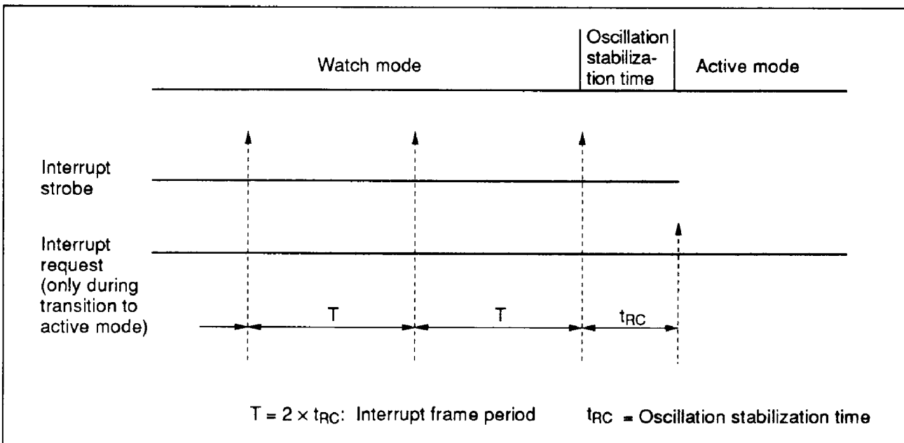
Figure 14 Interrupt Frame
