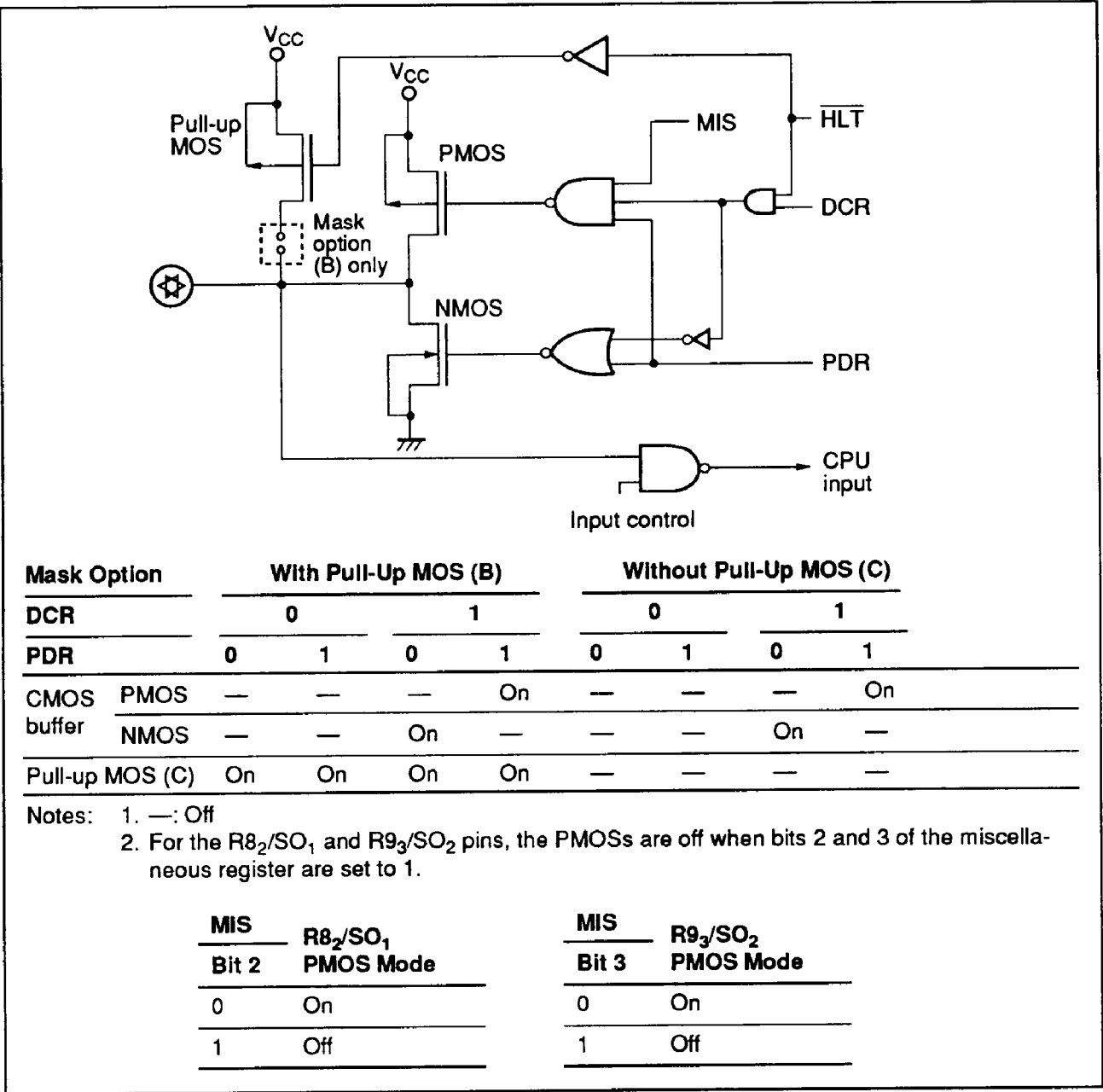
Figure 21 Input/Output Buffer
