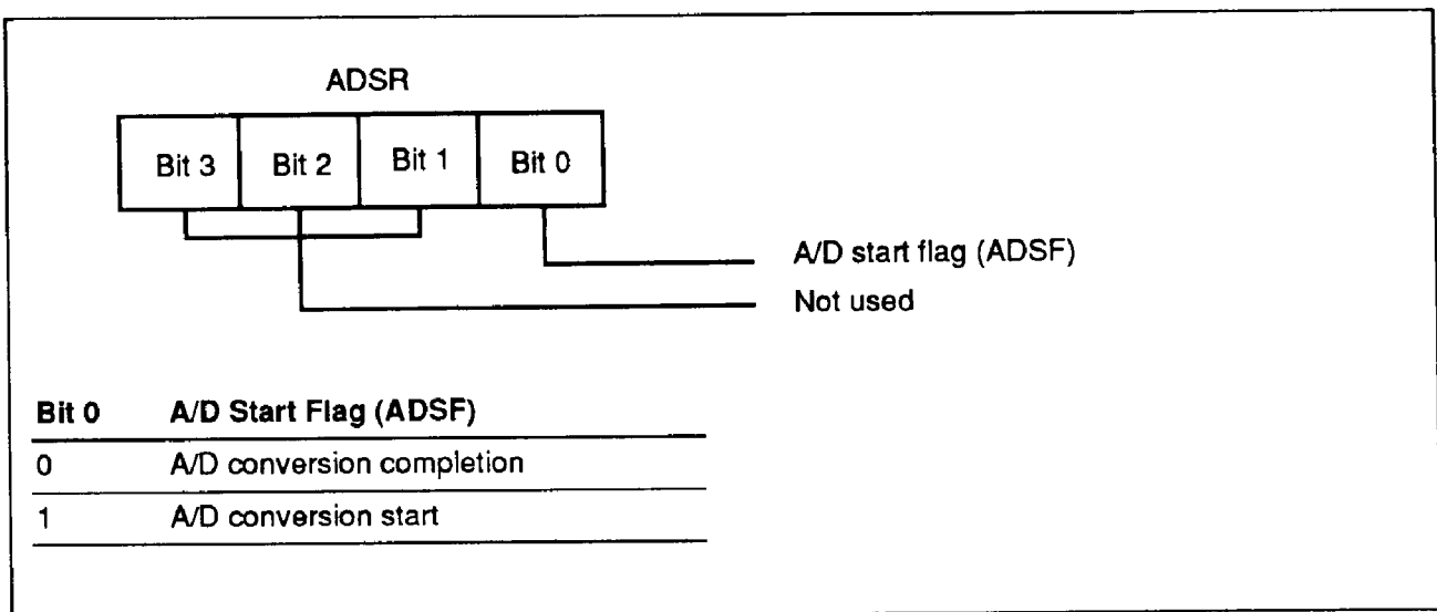
Figure 54 A/D Status Register
