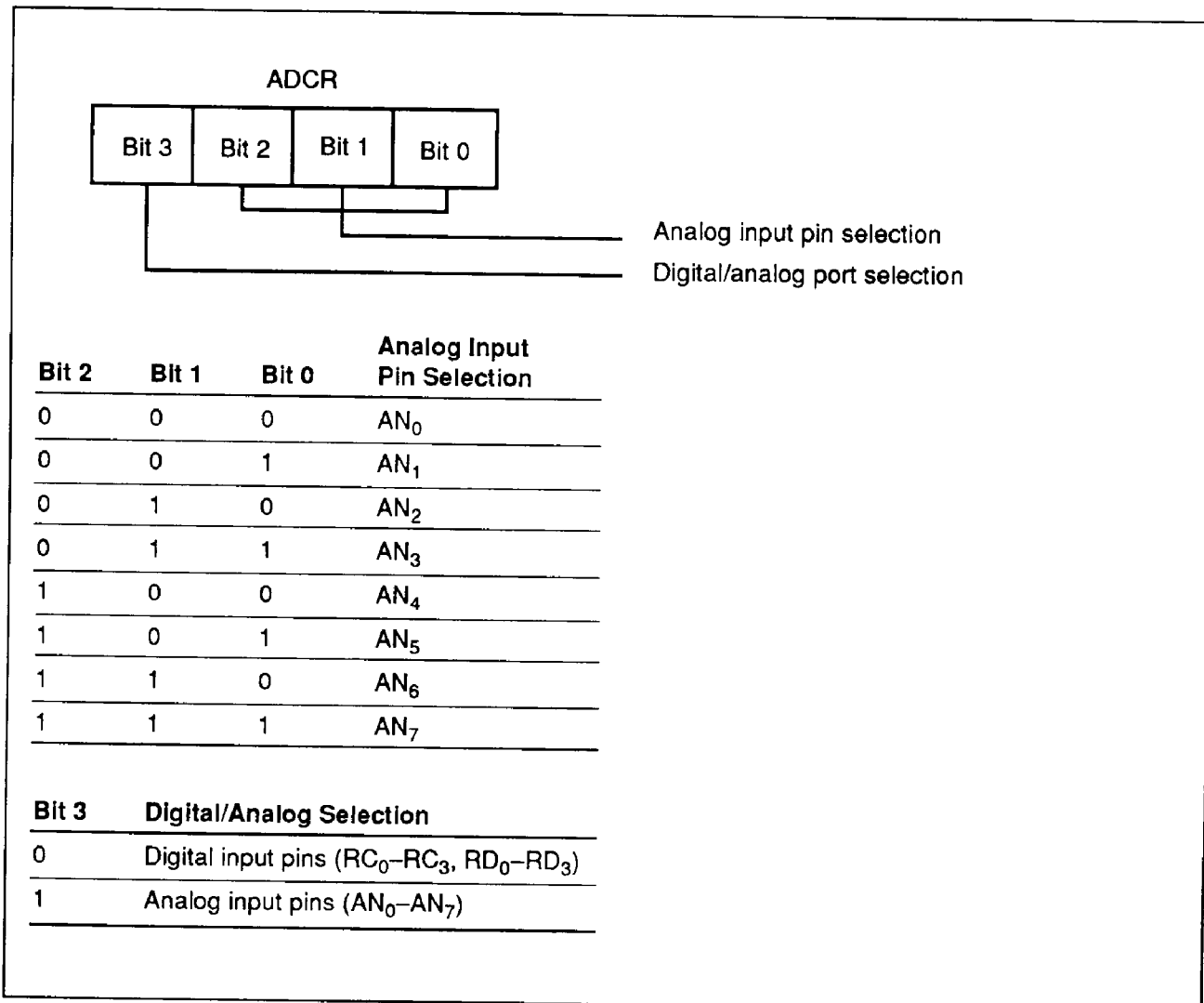
Figure 52 A/D Control Register
