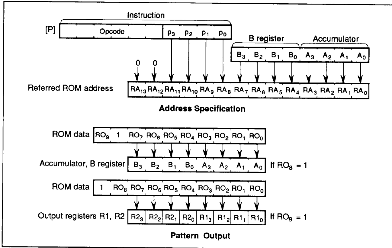
Figure 66 P Instruction
