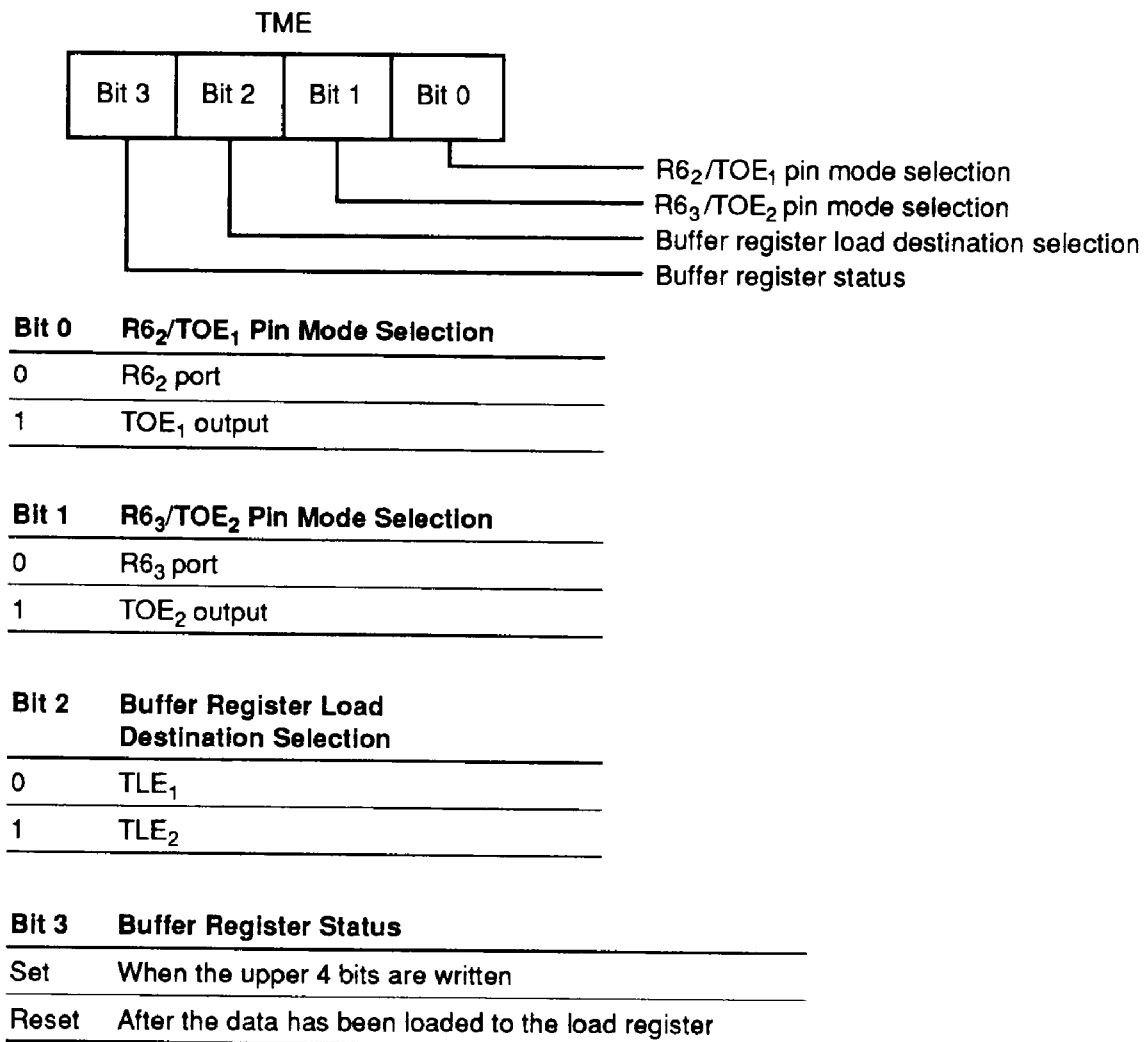
Figure 31 Timer Mode Register E
