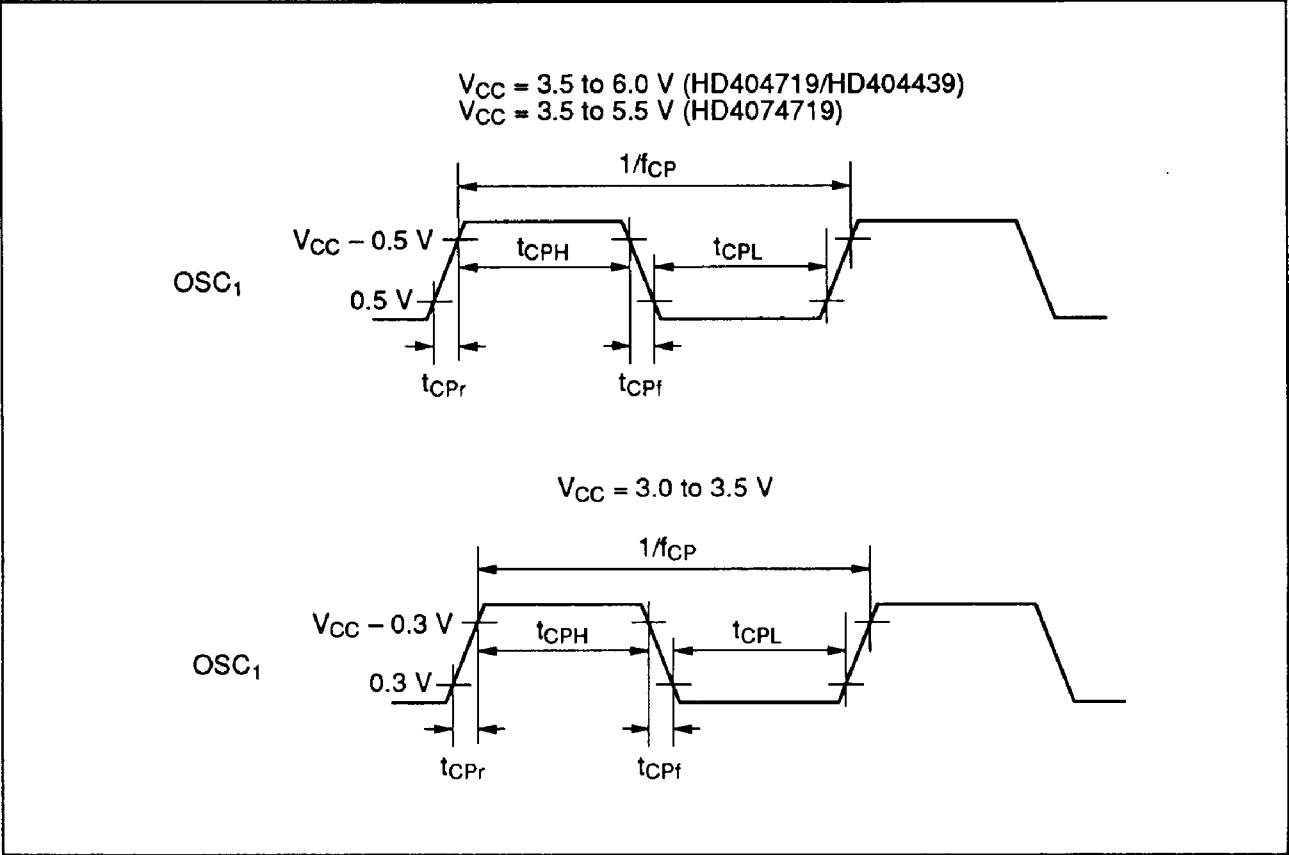
Figure 70 Oscillator Waveforms
