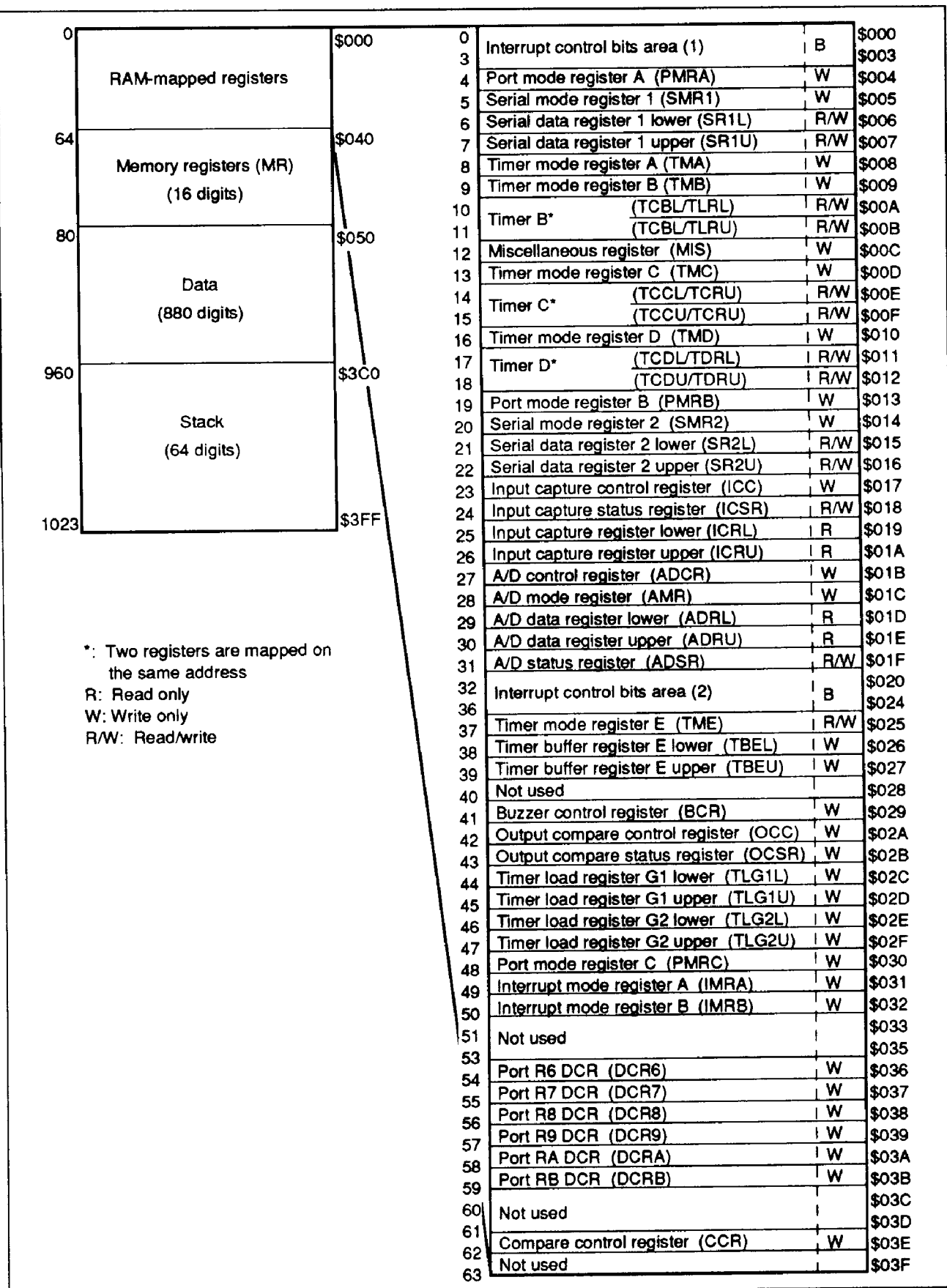
Figure 2 RAM Memory Map
