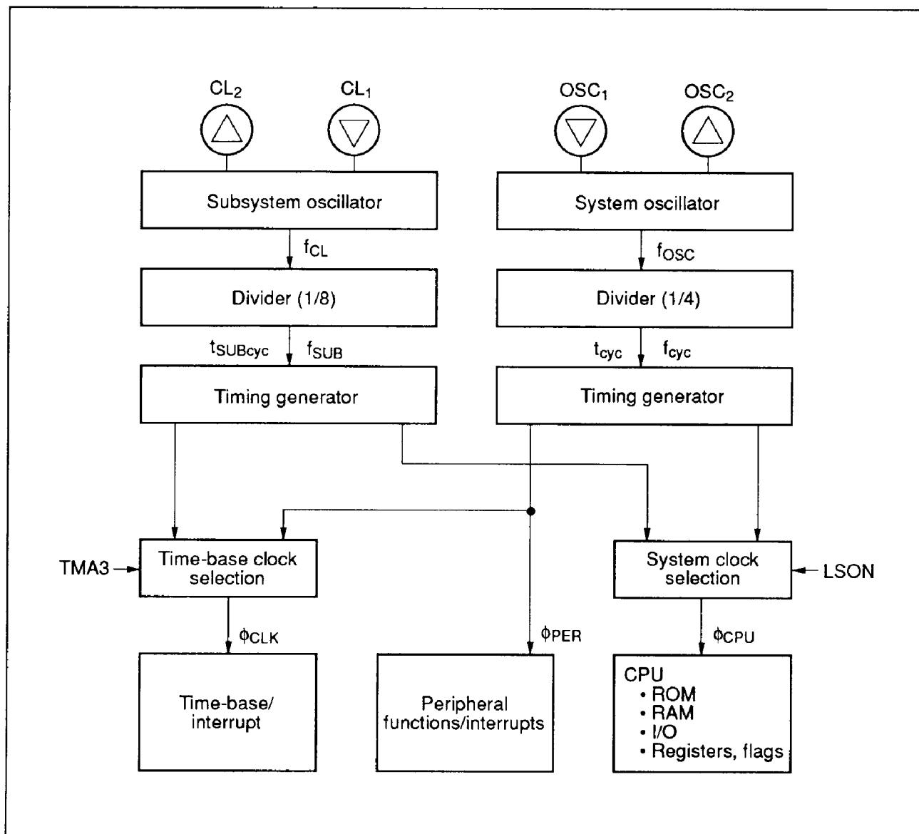
Figure 19 Internal Oscillation Circuit
