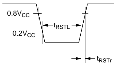
Figure 53 \overline{\text{RESET}} Timing
