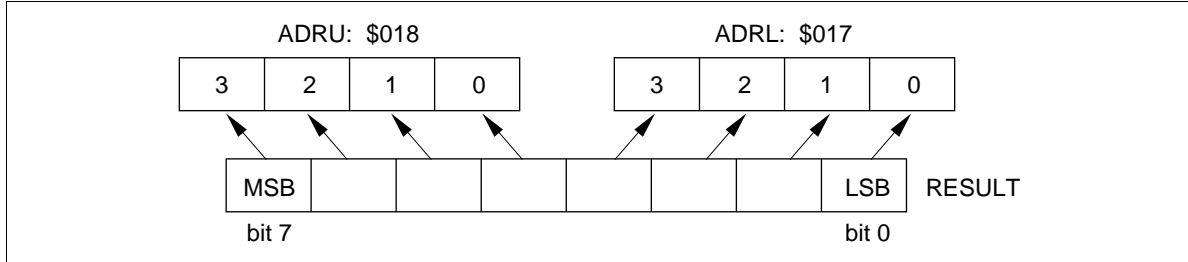
Figure 46 A/D Data Registers
