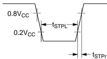
Figure 54 \overline{\text{STOPC}} Timing
