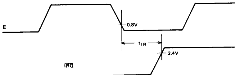
Figure 3 \overline{IR\bar{O}} Release Time
