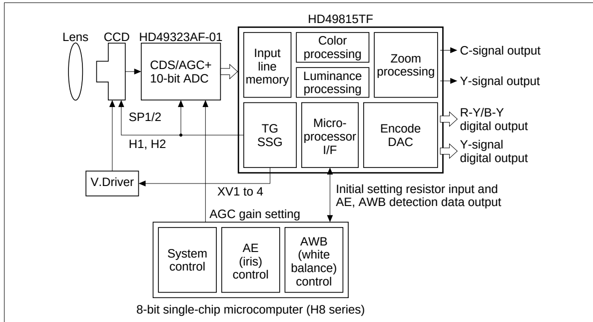
Figure 2 System Configuration
