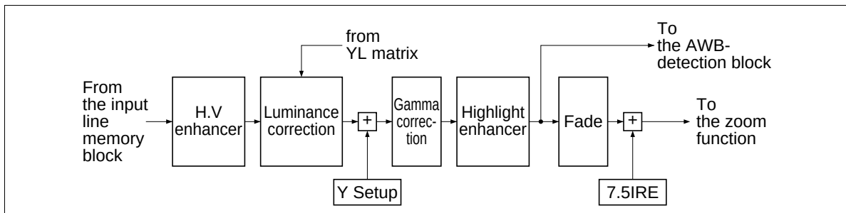
Figure 5 Luminance-Signal-Processing Block
