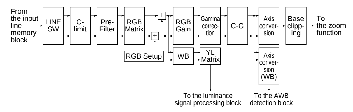
Figure 4 Color-Signal Processing Block
