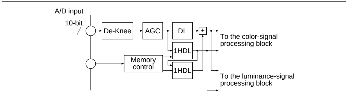
Figure 3 Input Line Memory Block
