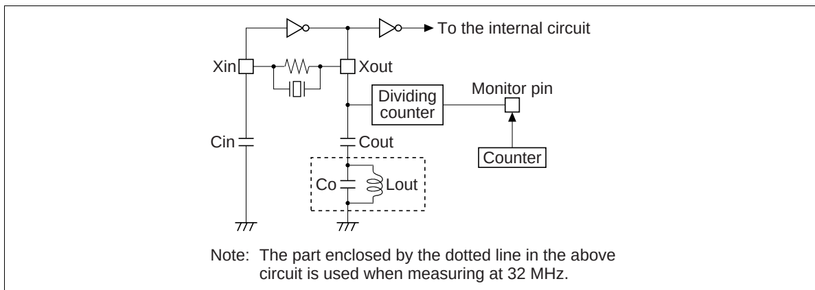
Figure 1 Measuring Circuit
