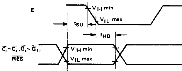
Figure 5 Input Setup and Hold Times
