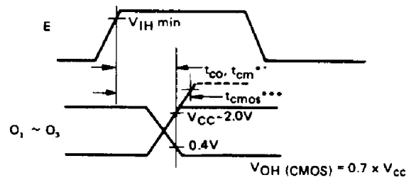
Figure 6 Output Delay
