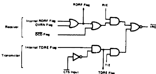
Figure 14 IRQ Internal Circuit
