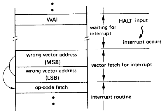
Figure 39 MAC function during WAI
