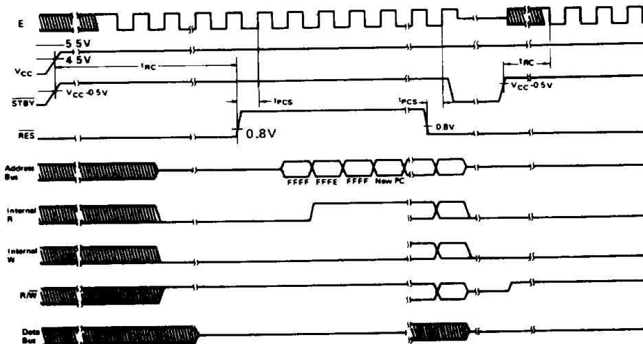
Figure 11 Reset Timing
