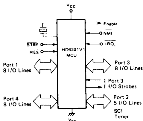
Figure 15 HD6301V1 MCU Single-Chip Mode
