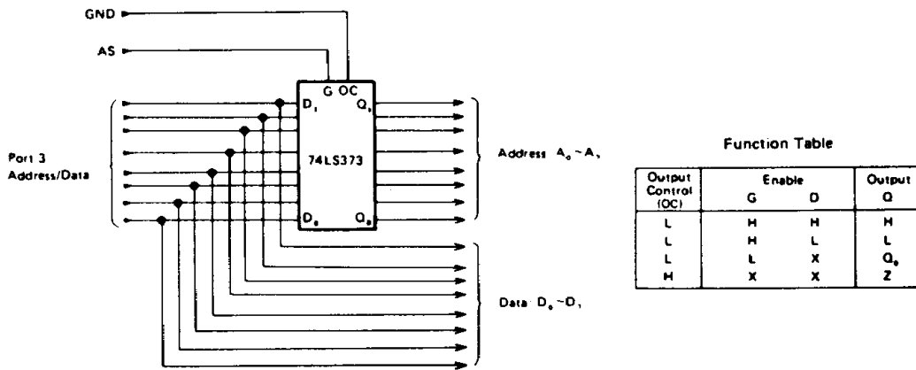
Figure 18 Latch Connection
