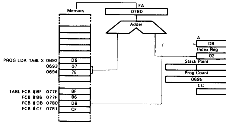
Figure 36 Example of Indexed (16-bit Offset) Addressing
