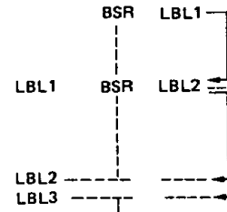
example of malfunction of 2nd BSR execution
