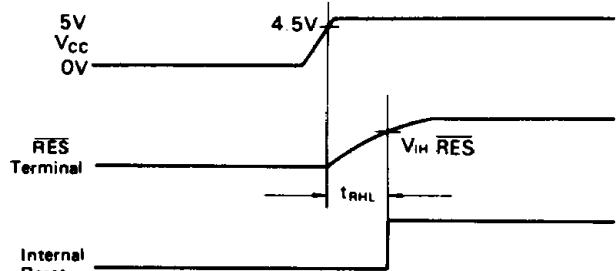
Figure 18 Power On and Reset Timing
