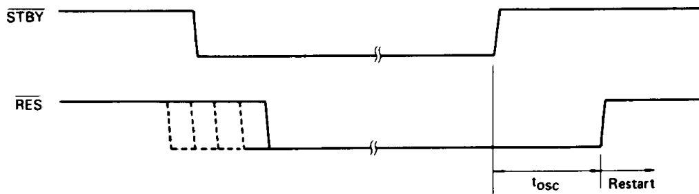
Figure 26 Timing Chart of Releasing from Standby Mode
