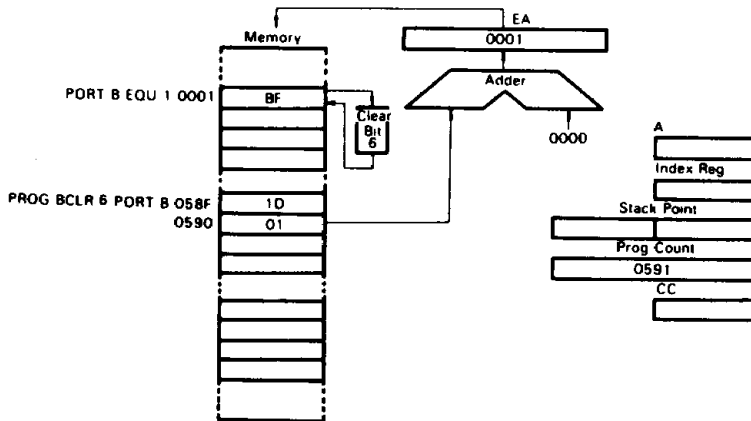
Figure 37 Example of Bit Set/Clear Addressing
