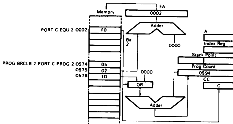
Figure 38 Example of Bit Test and Branch Addressing
