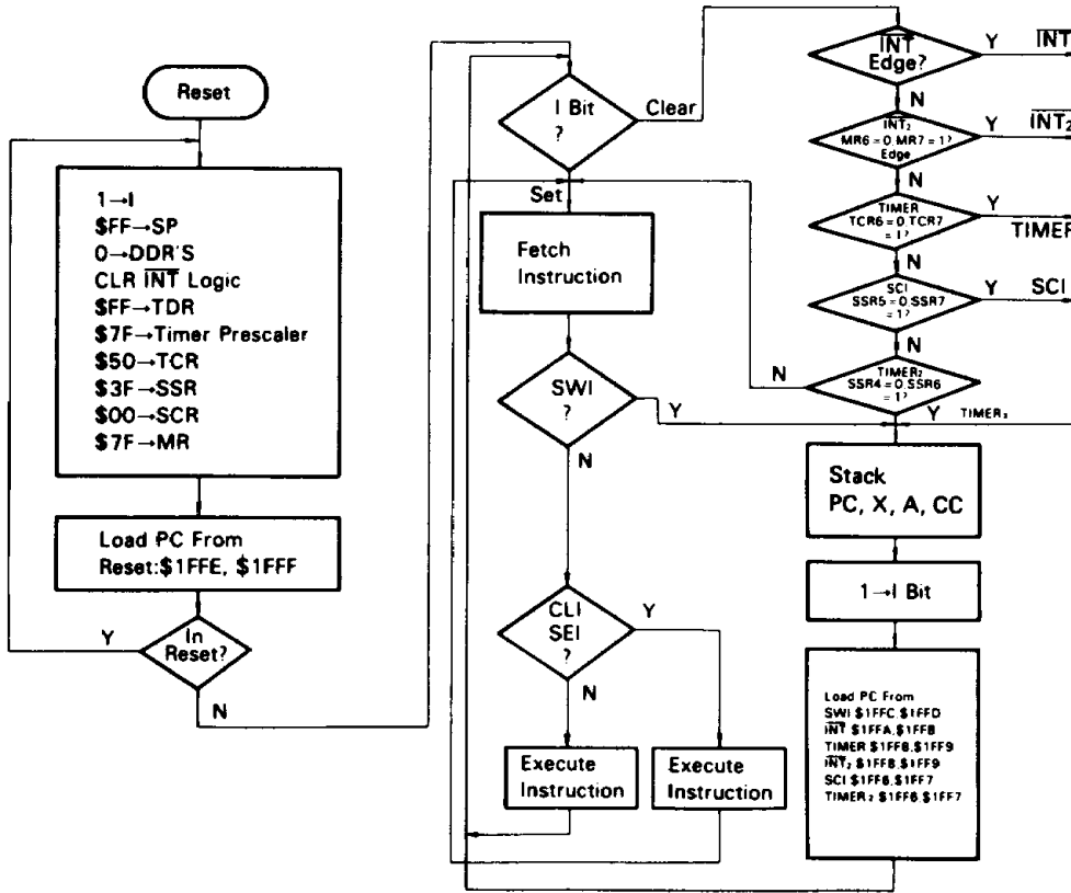
Figure 12 Interrupt Flowchart
