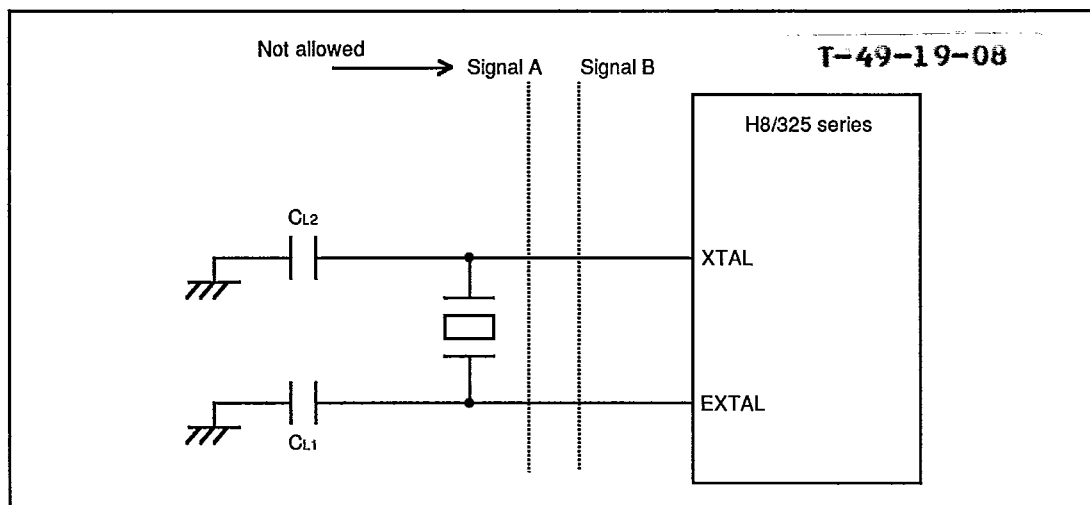
Figure 14-4. Notes on Board Design around External Crystal
