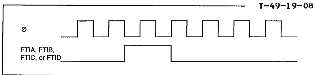
Figure 7-2. Minimum Input Capture Pulse Width (Noise Canceller Disabled)
