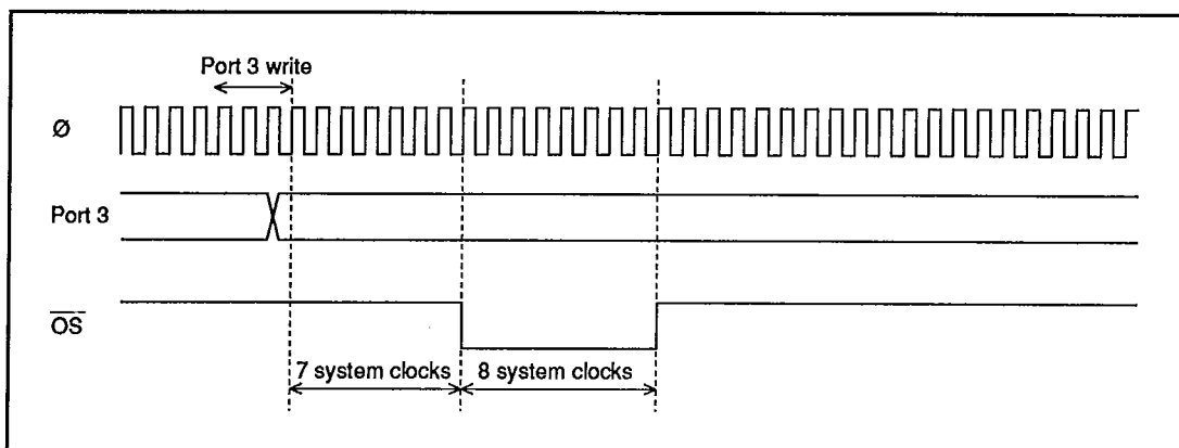
Figure 6-2. Output Strobe Output Timing (When OSS = 1)
