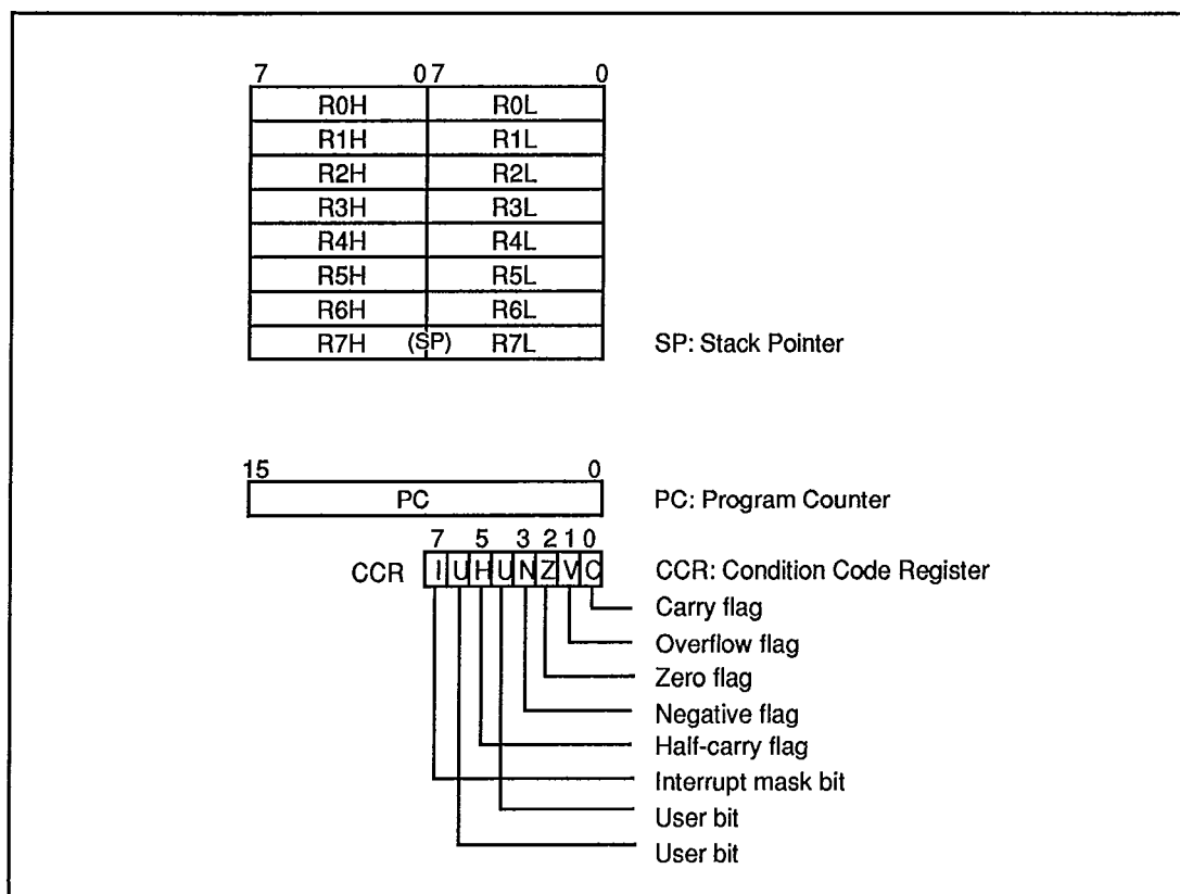
Figure 3-1. CPU Registers
