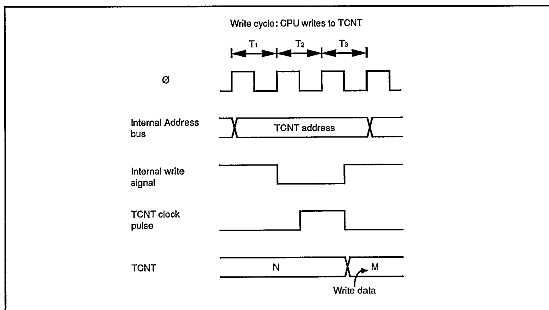
Figure 8-14. TCNT Write-Increment Contention
