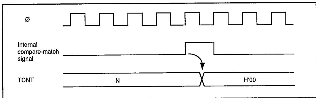
Figure 8-8. Timing of Compare-Match Clear
