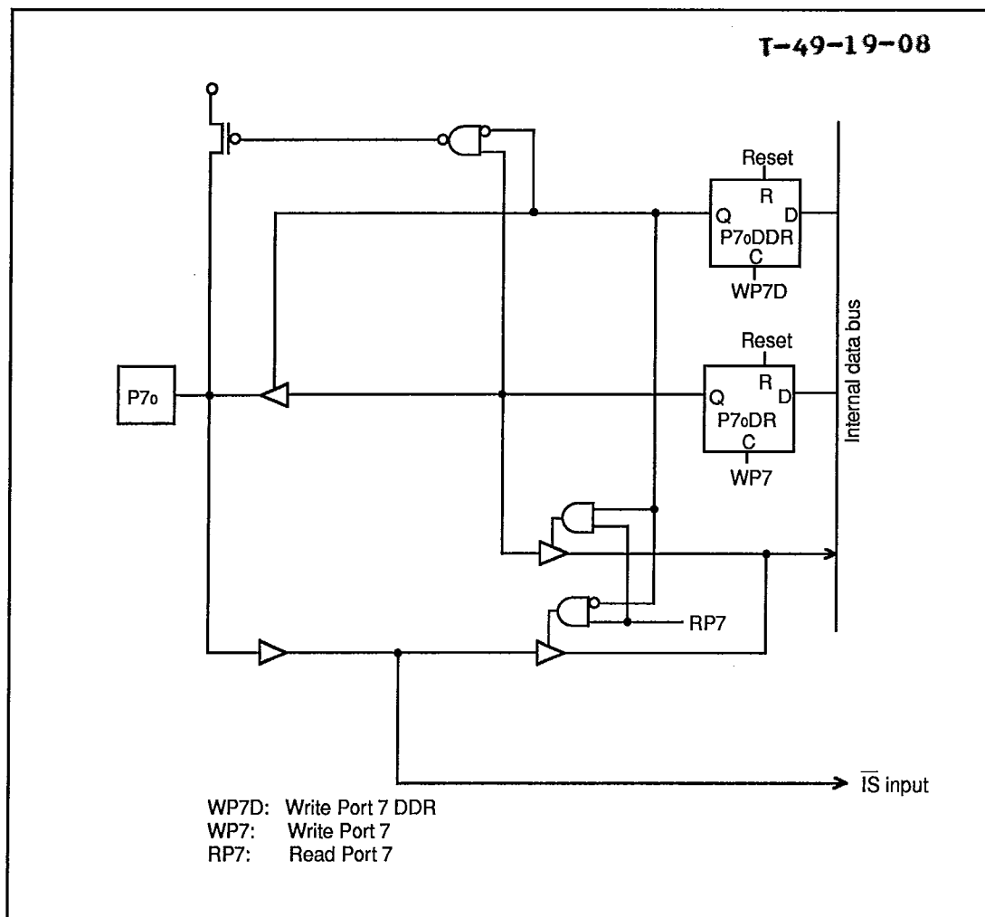
Figure 5-14. Port 7 Schematic Diagram (Pin P70)
