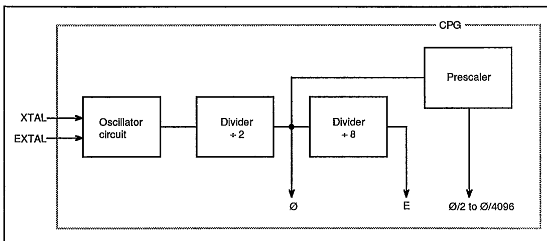
Figure 14-1. Block Diagram of Clock Pulse Generator
