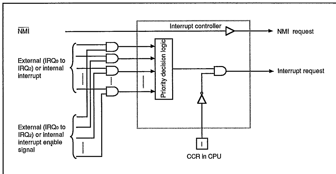
Figure 4-3. Block Diagram of Interrupt Controller
