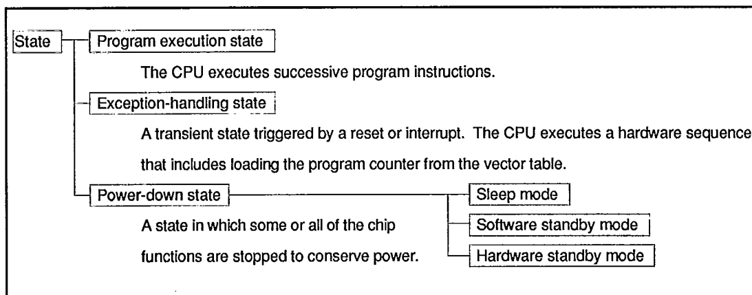
Figure 3-11. Operating States
