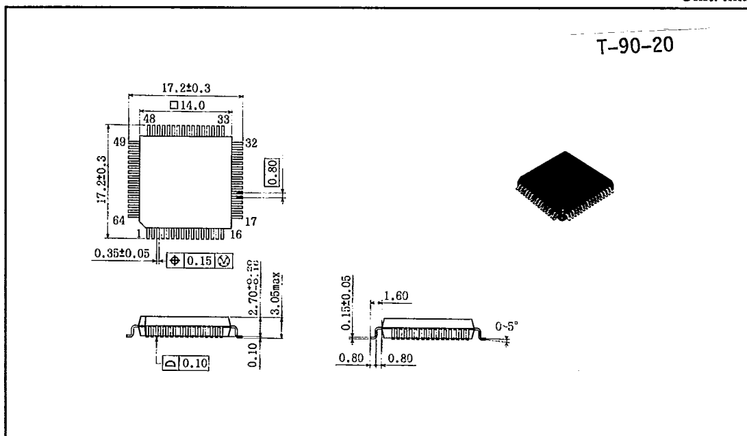
Figure E-3. Package Dimensions (FP-64A)
