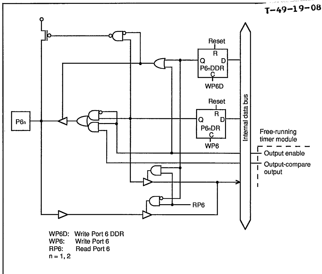
Figure 5-12. Port 6 Schematic Diagram (Pins P61 and P62)
