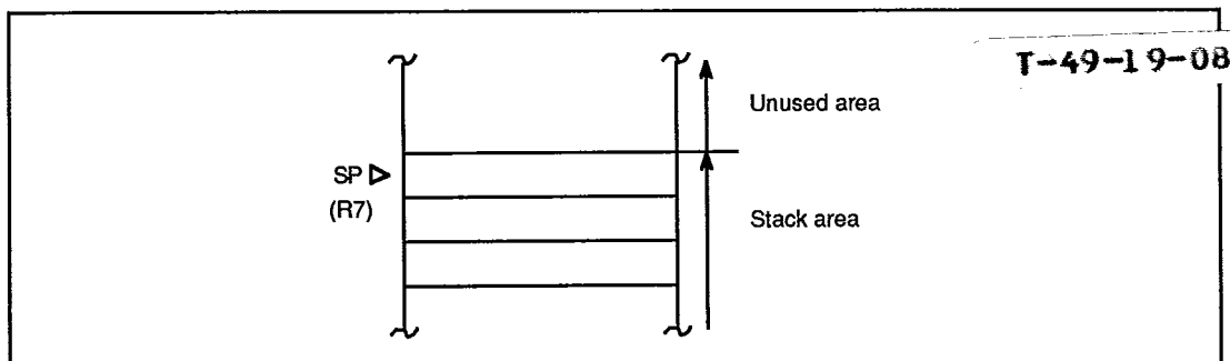
Figure 3-2. Stack Pointer
