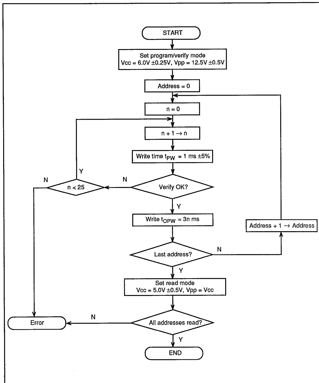
Figure 11-6. High-Speed Programming Flowchart
