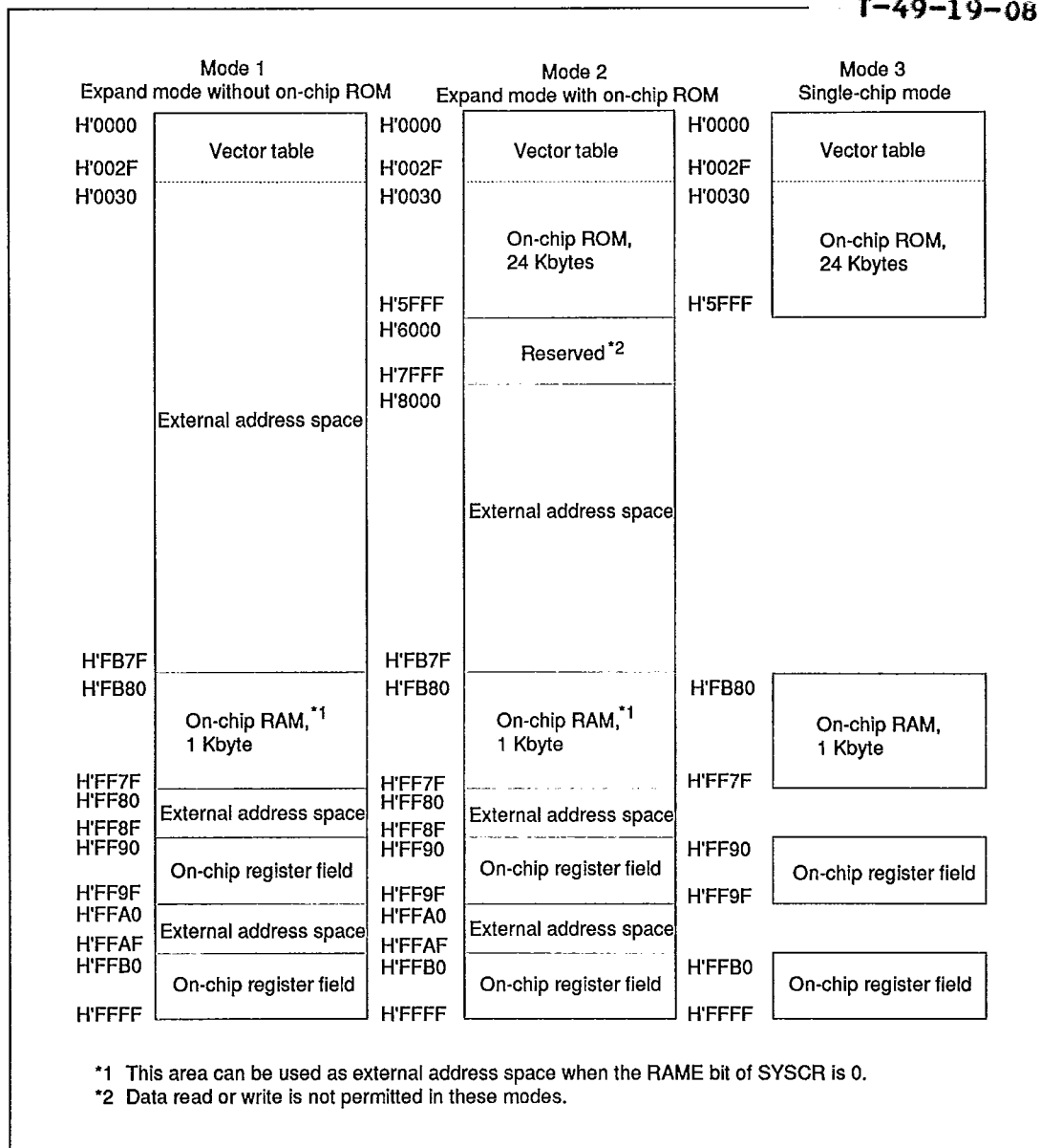
Figure 2-2. H8/324 Address Space Map
