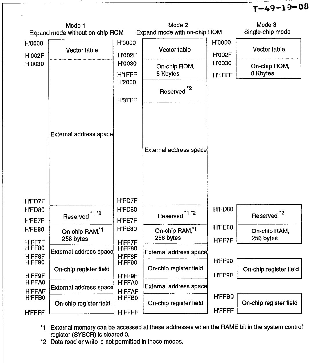
Figure 2-4. H8/322 Address Space Map
