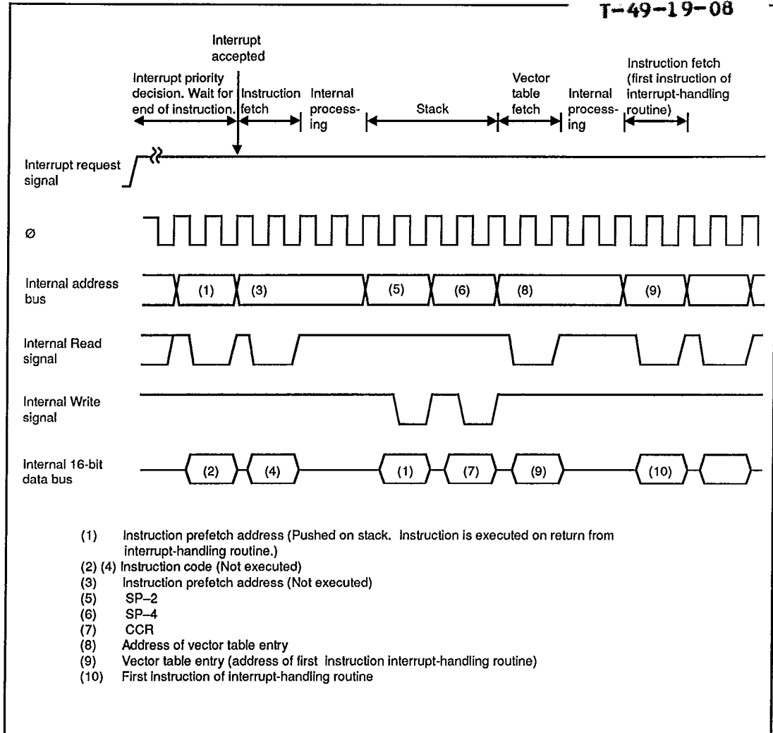
Figure 4-6. Timing of Interrupt Sequence
