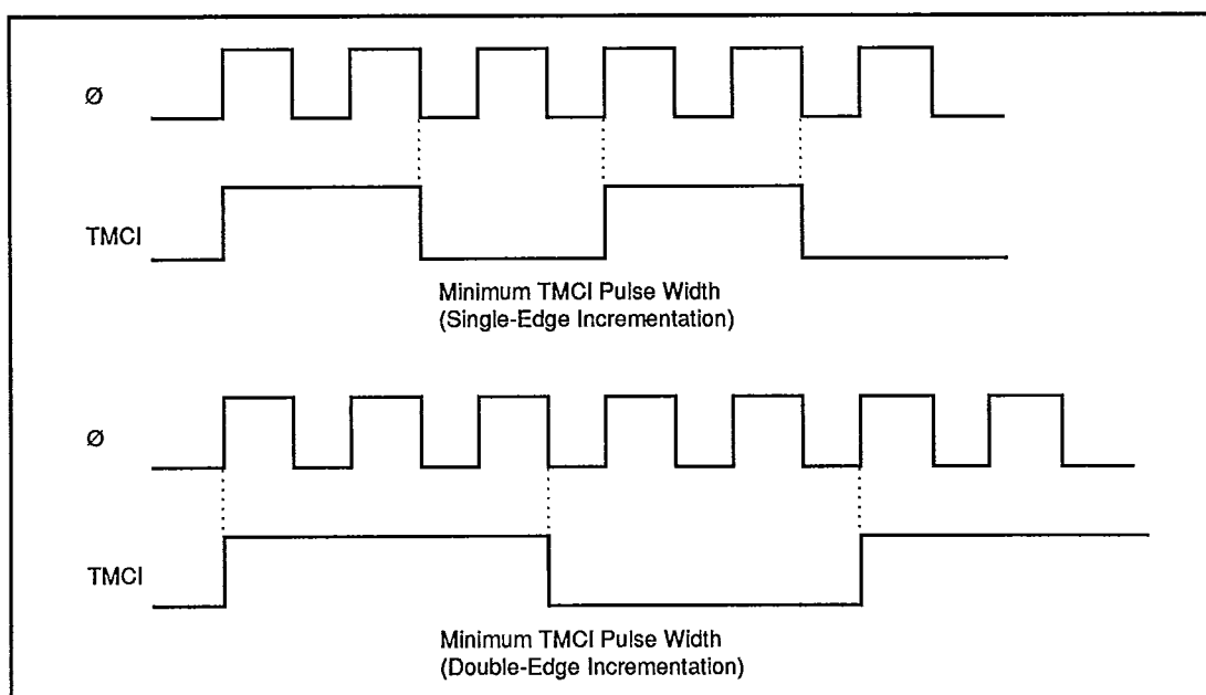
Figure 8-4. Minimum External Clock Pulse Widths (Example)
