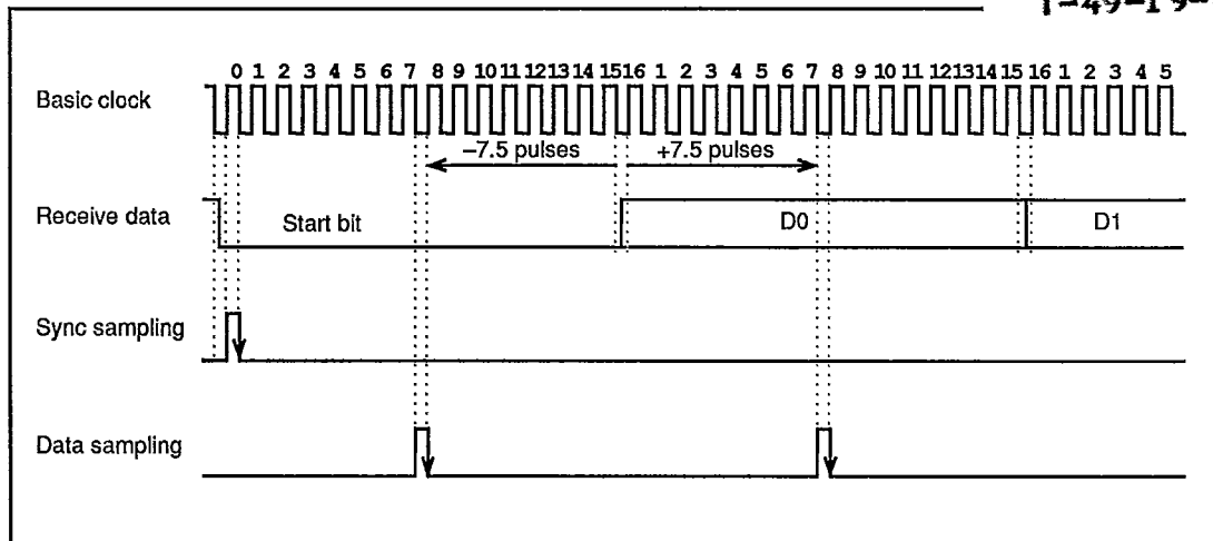
Figure 9-5. Sampling Timing (Asynchronous Mode)
