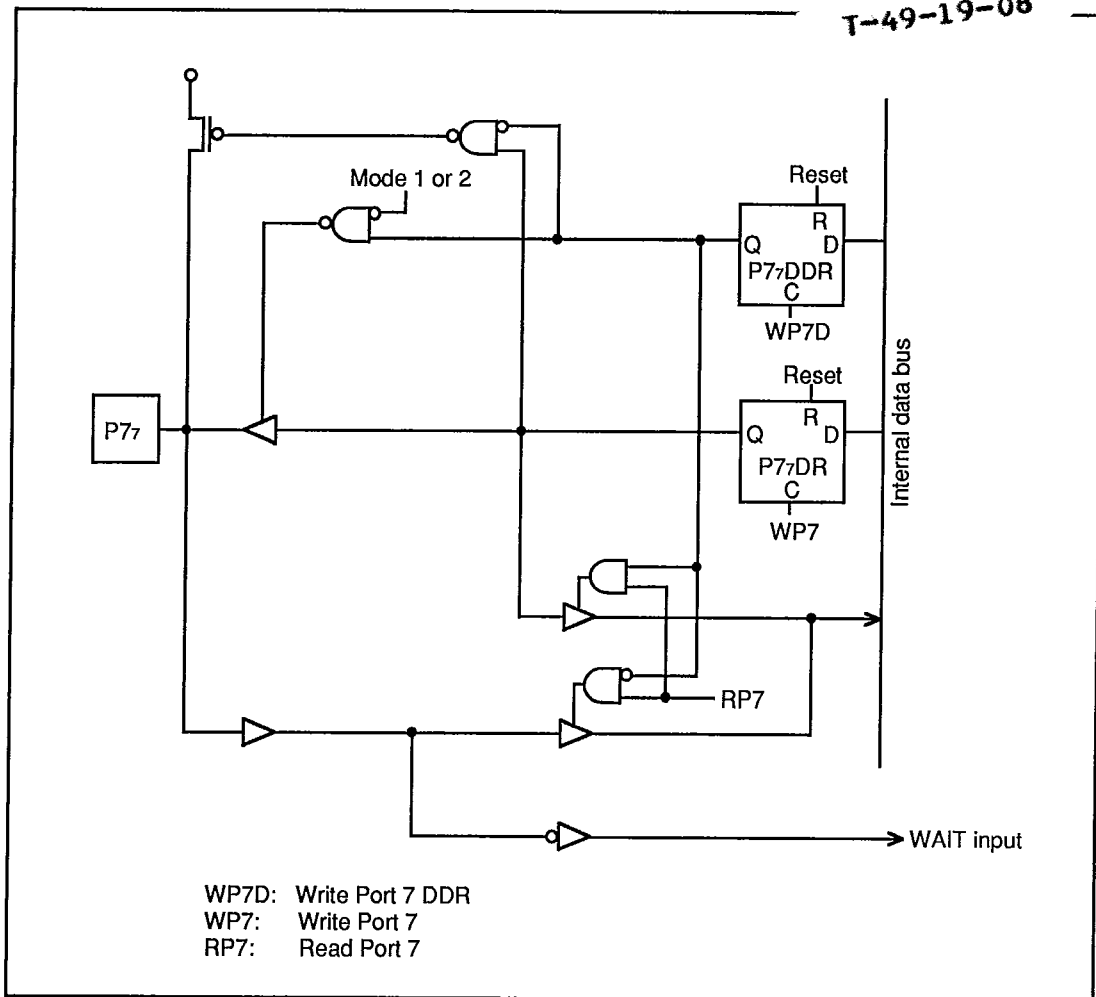
Figure 5-18. Port 7 Schematic Diagram (Pin P77)
