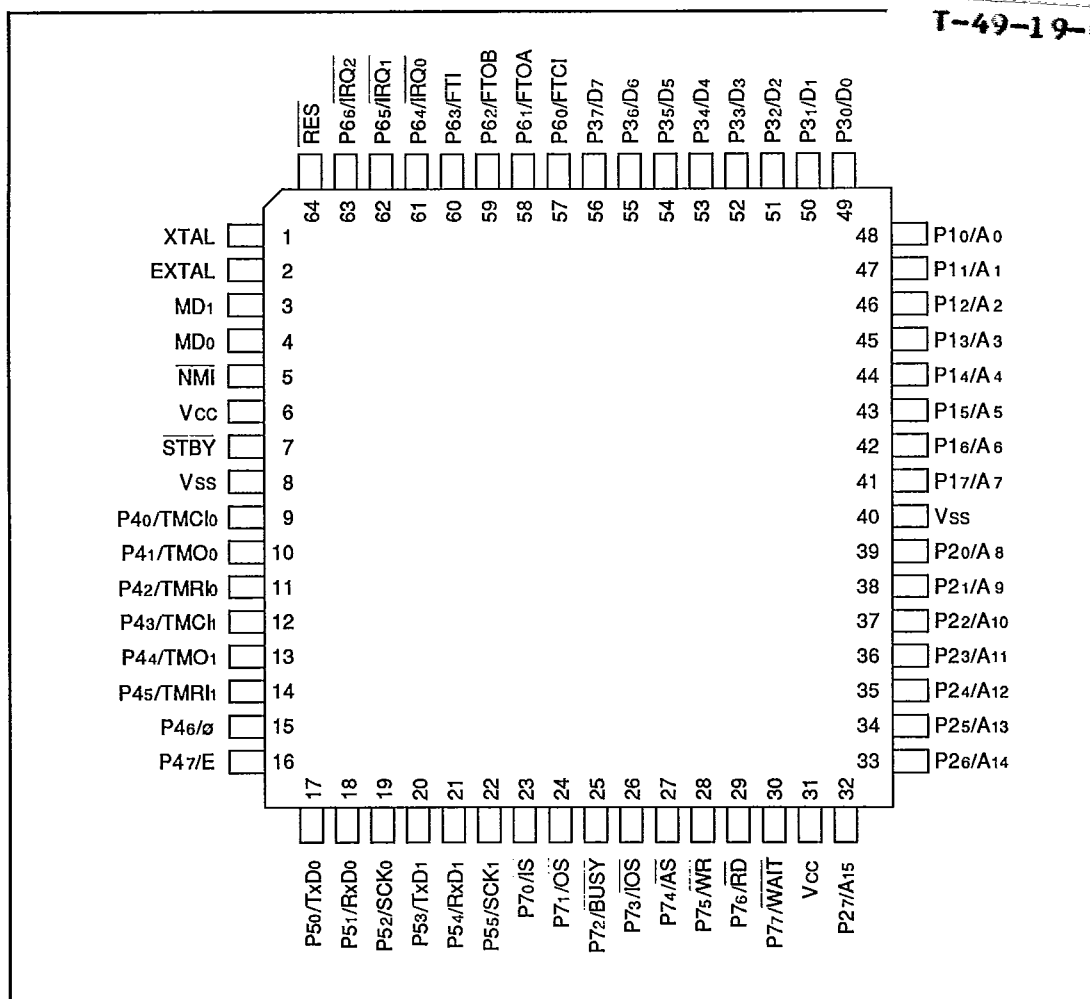
Figure 1-3. Pin Arrangement (FP-64A, Top View)
