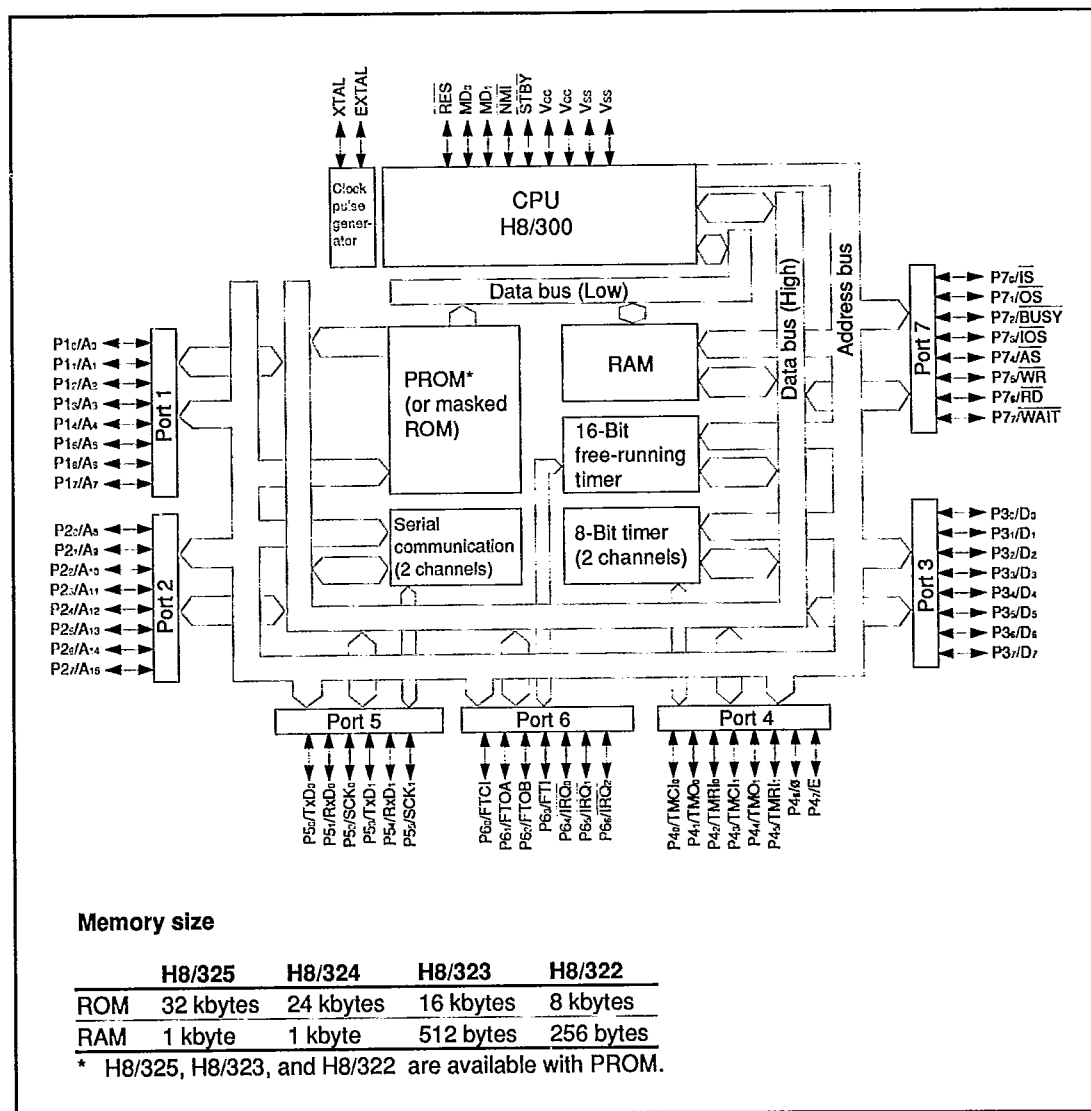
Figure 1-1. Block Diagram
