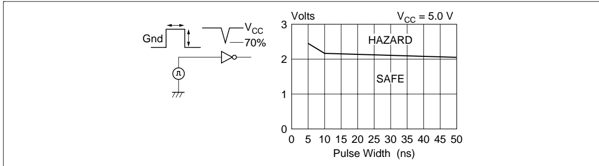
Figure 14 Low Noise Margin
