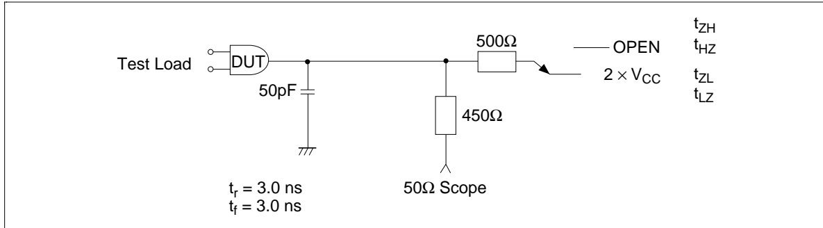
Figure 1 AC Loading Circuit
