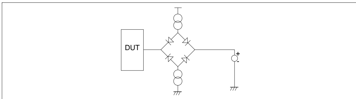
Figure 26 MCT Wheatstone Bridge Test Load
