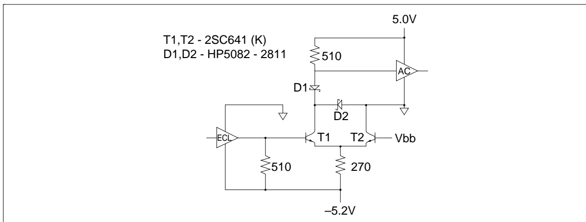
Figure 5 Single-Ended ECL-to-HD74AC Circuit
