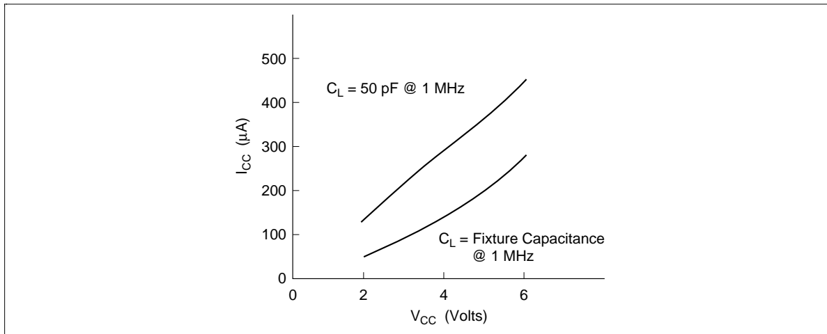
Figure 1 I_{CC} vs V_{CC}
