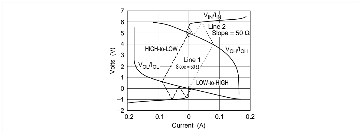
Figure 2 Gate Driving 50\ \Omega Line Reflection Diagram
