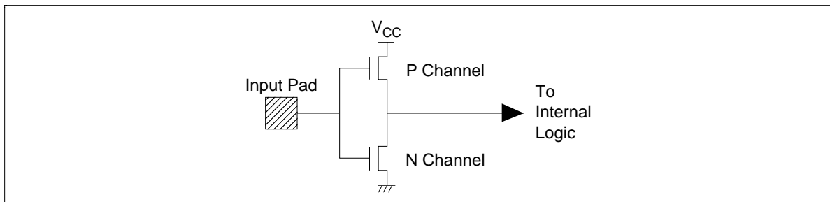
Figure 20 CMOS Input Structure
