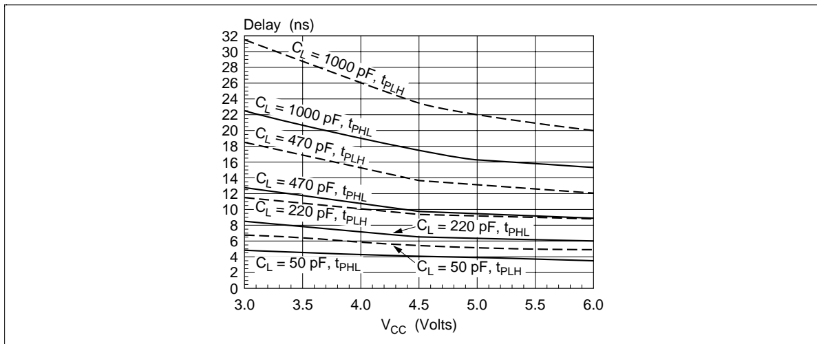
Figure 11 Propagation Delay vs. V_{CC} (HD74AC00)
