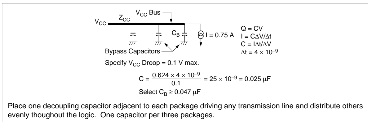
Figure 19 Formula for Calculating Decoupling Capacitors
