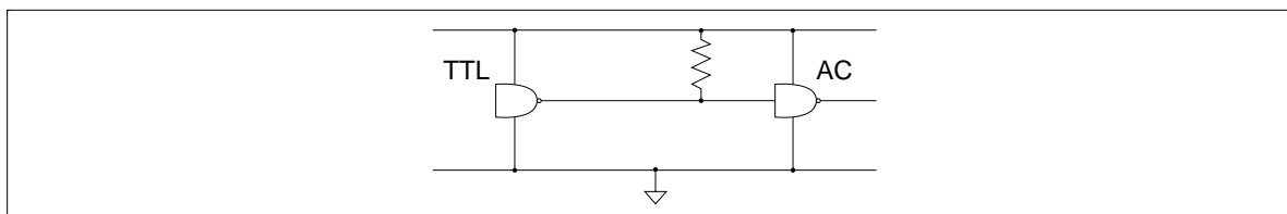
Figure 2 V_{IH} Pull-Up on TTL Outputs
