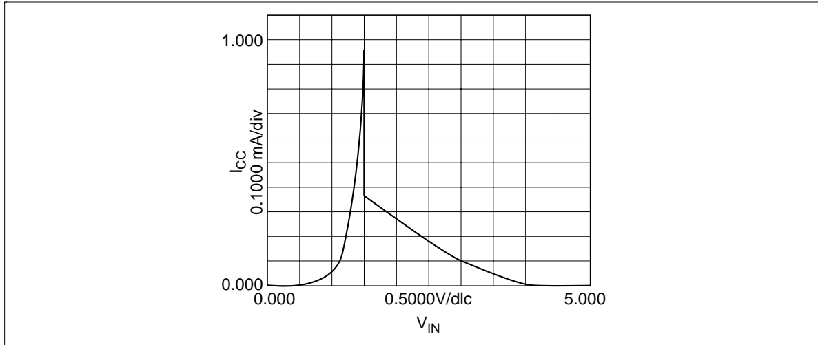
Figure 21 I_{CC} versus Input Voltage for HD74ACT Devices
