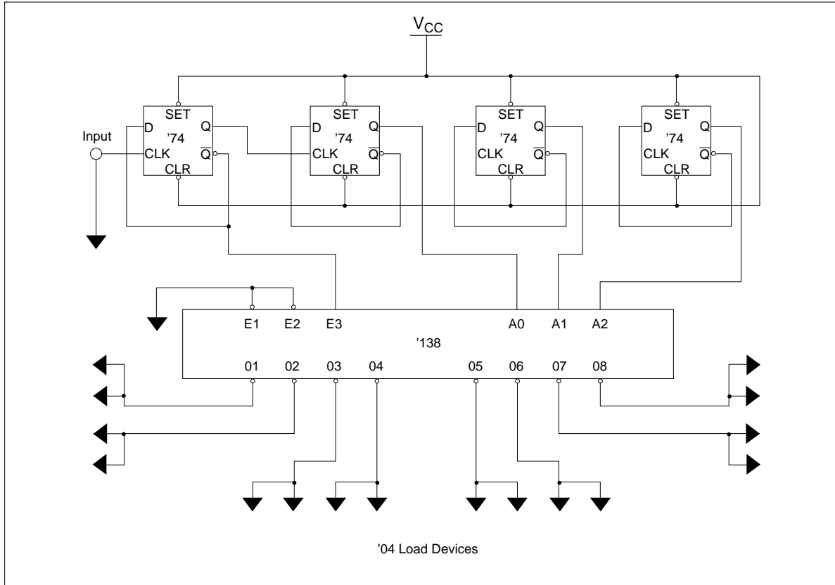
Figure 9 Power Demonstration Circuit Schematic
