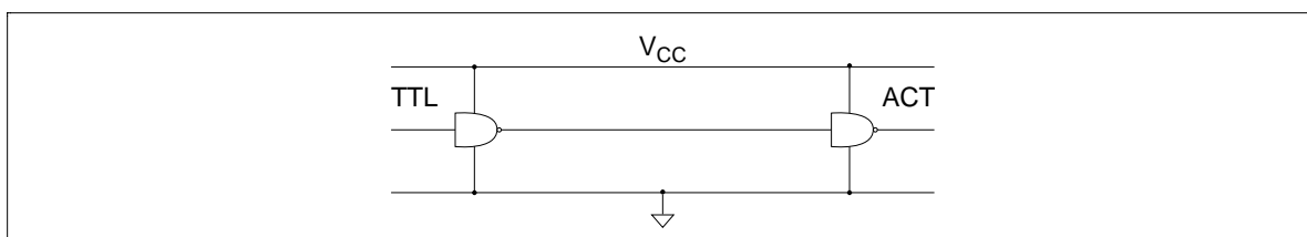
Figure 3 TTL Interfacing to HD74ACT
