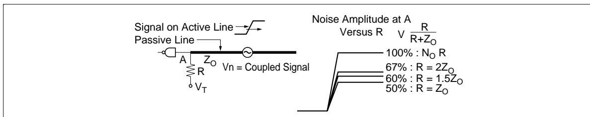
Figure 15 Effects of Termination on Crosstalk
