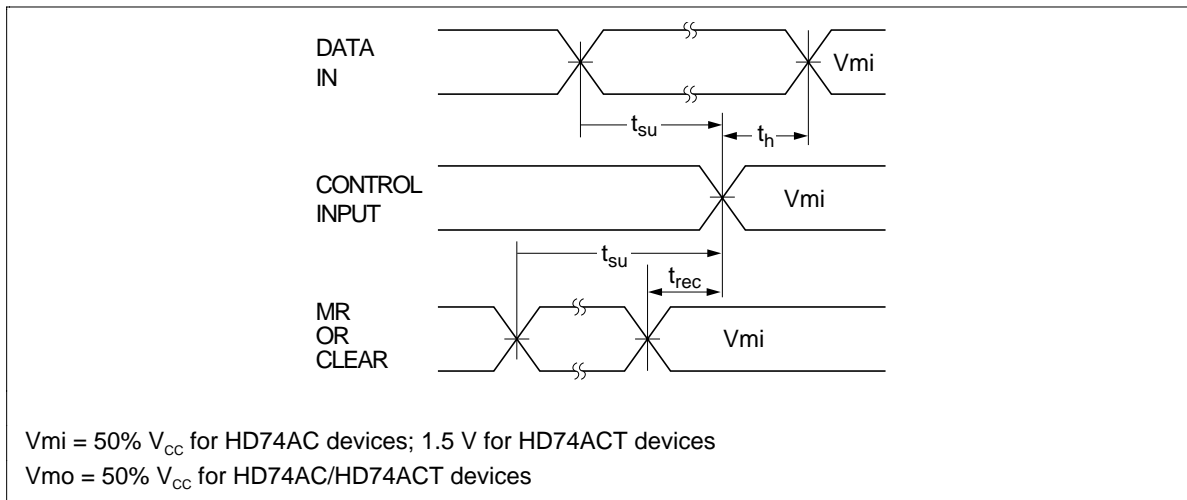
Figure 7 Setup Time, Hold Time and Recovery Time
