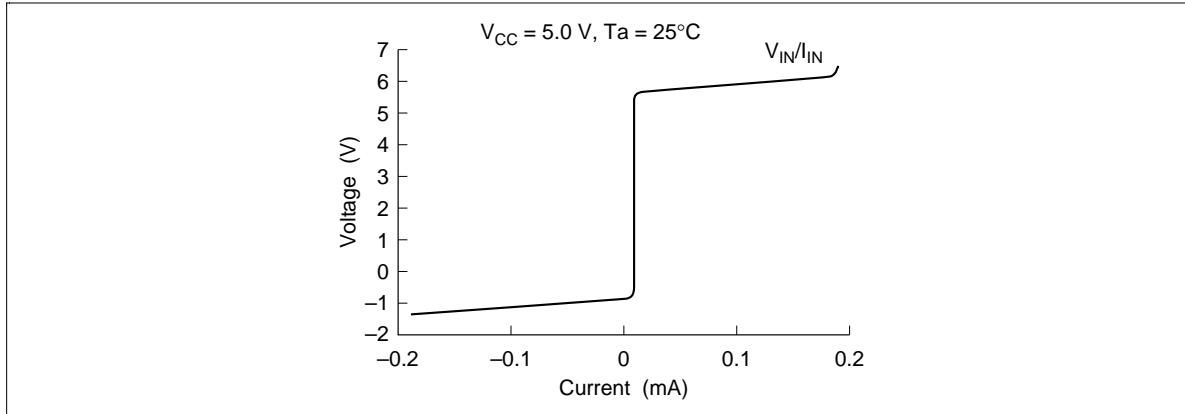
Figure 7 Input Characteristics V_{IN}/I_{IN}
