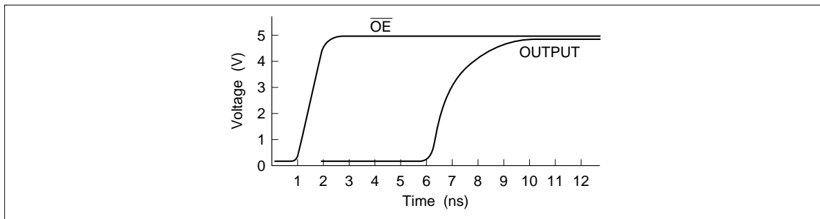
Figure 25 Typical Bench 3-State Waveform
