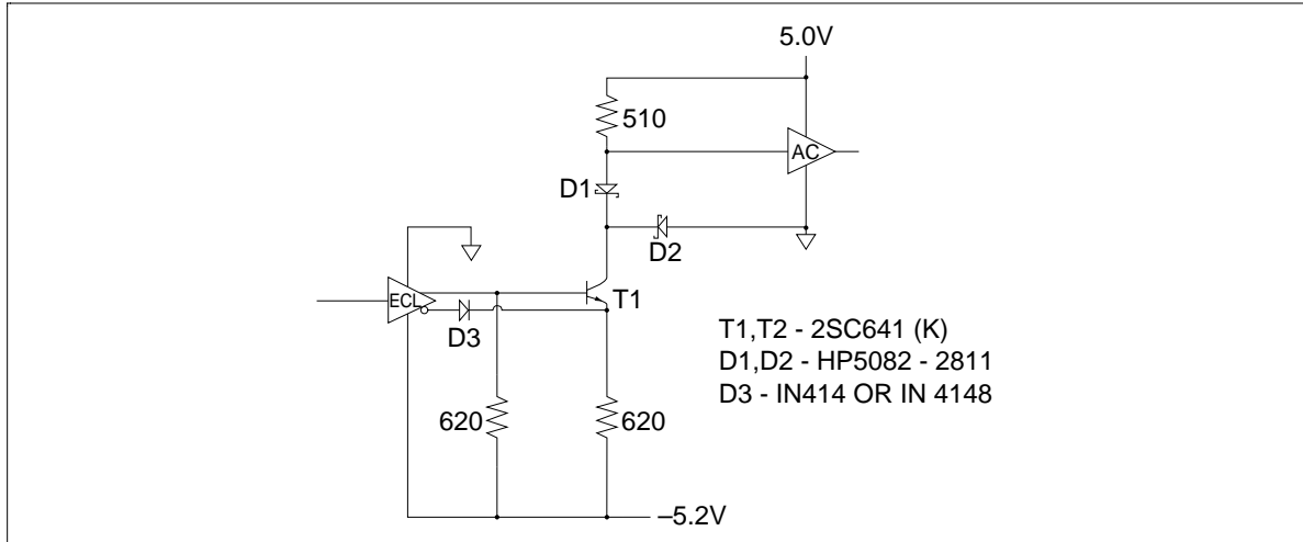
Figure 6 Differential Output ECL-to-HD74AC Circuit
