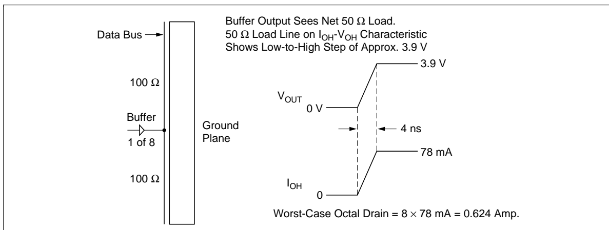
Figure 18 Octal Buffer Driving a 100 Ω Bus
