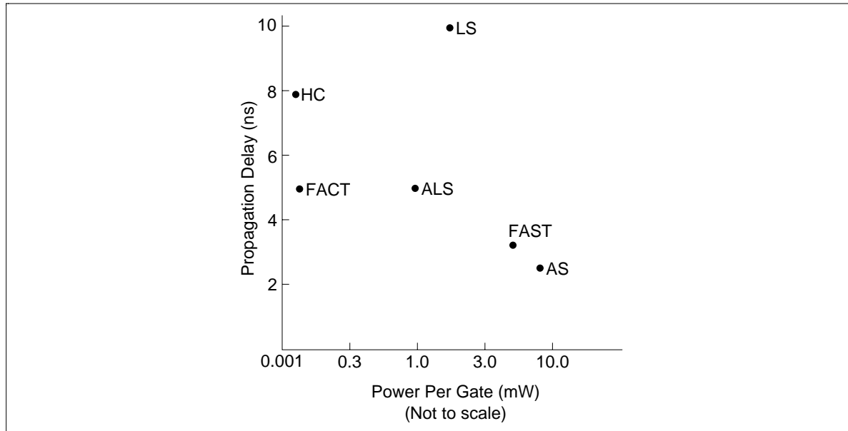
Figure8 Propagation Delays
