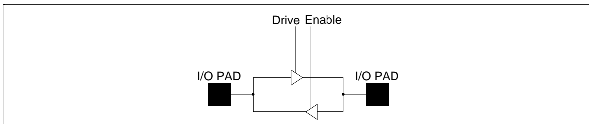
Figure 23 HD74AC245/HD74ACT245 I/O Structure
