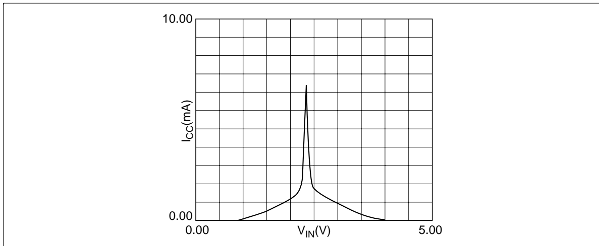
Figure 22 I_{CC} versus V_{IN}
