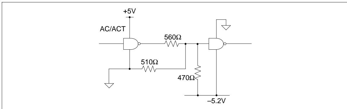
Figure 4 Resistive FACT-to-ECL Translation
