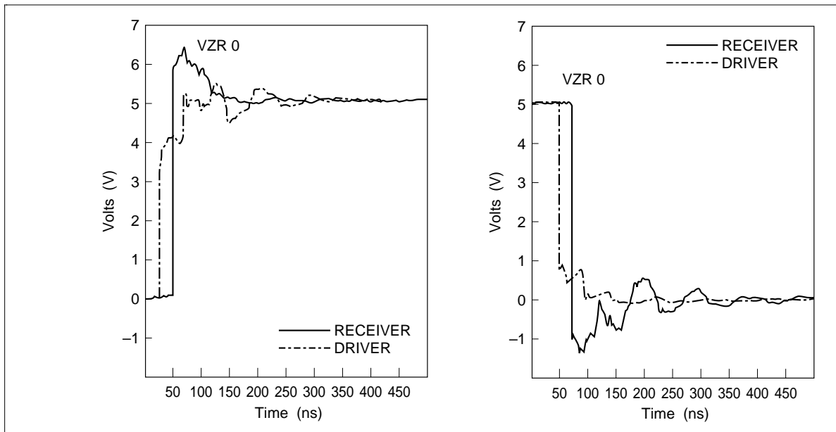
Figure 4 Resultant Waveforms Driving 50 Ω Line—Actual
