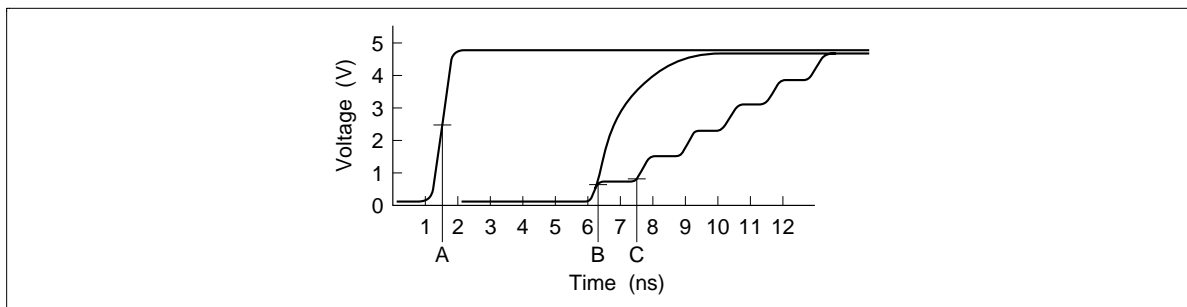
Figure 28 Measurement Stepout
