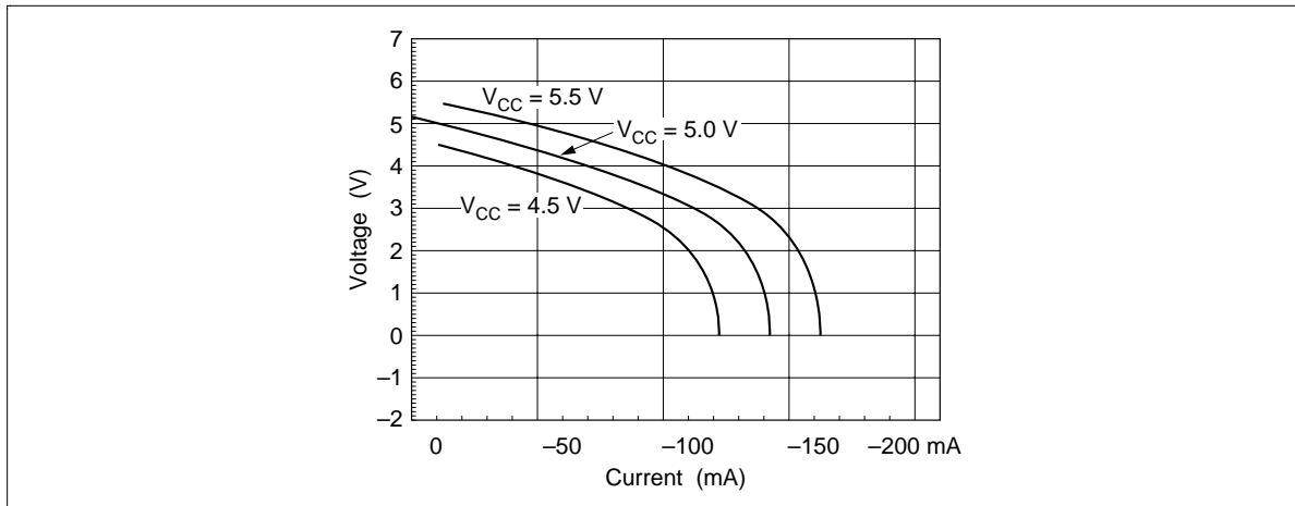
Figure 5 Output Characteristics V_{OH}/I_{OH} , HD74AC00
