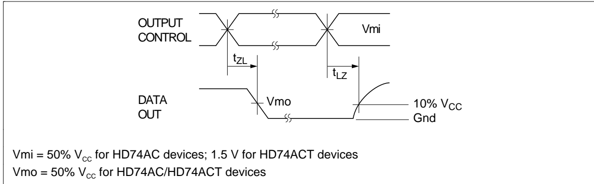
Figure 6 3-State Output Low Enable and Disable Times
