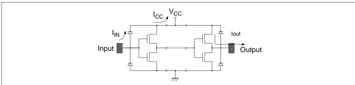
Figure 10 Clamp Diode Operation
