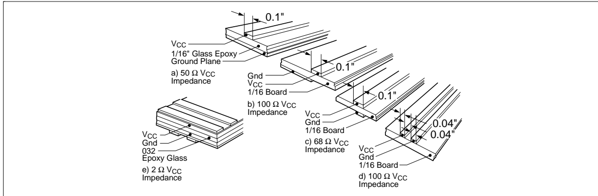
Figure 17 Power Distribution Impedances
