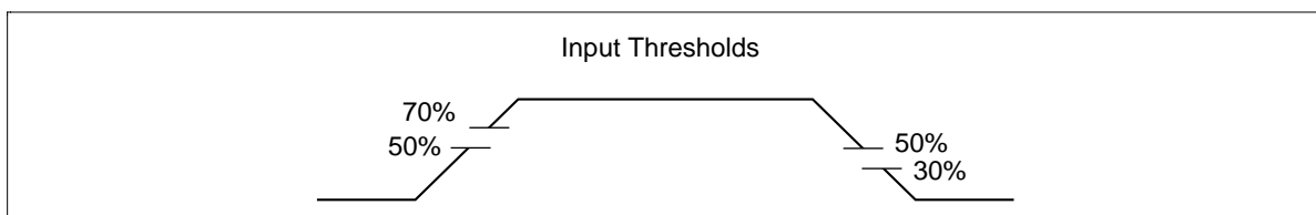
Figure 9 Input Threshold
