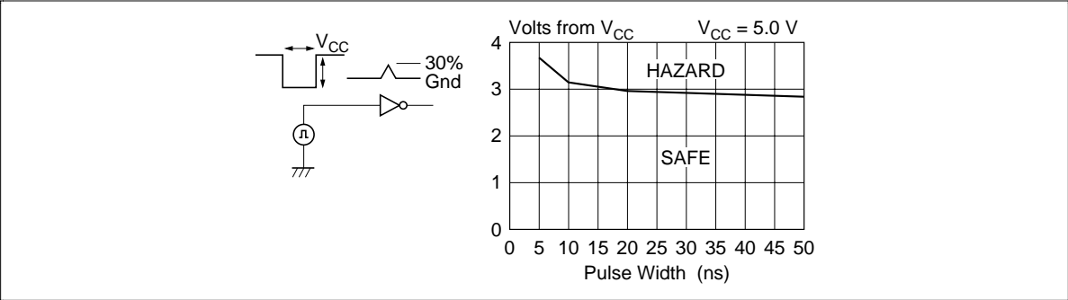
Figure 13 High Noise Margin
