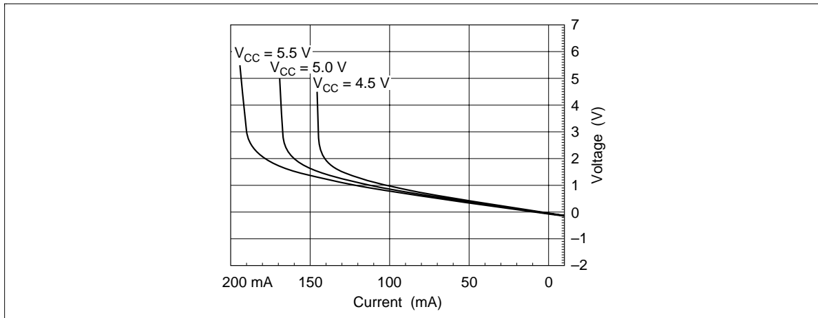
Figure 6 Output Characteristics V_{OL}/I_{OL} , HD74AC00
