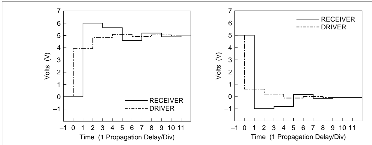
Figure 3 Resultant Waveforms Driving 50 Ω Line—Theoretical
