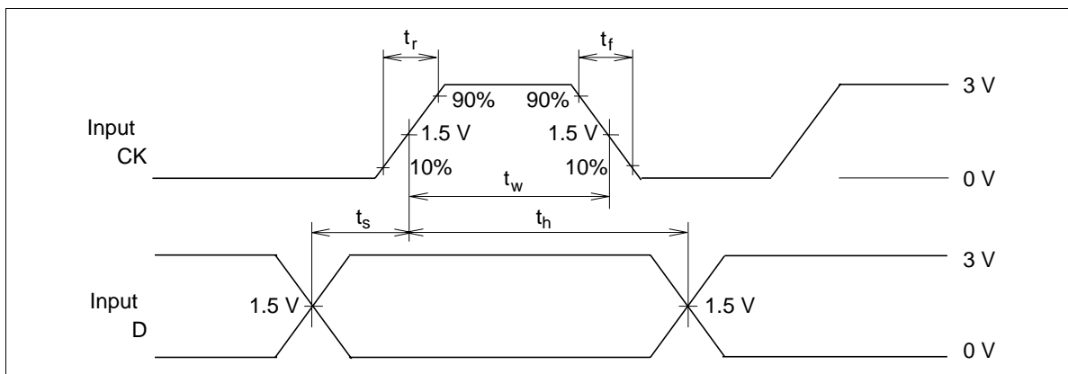
Waveforms-2
