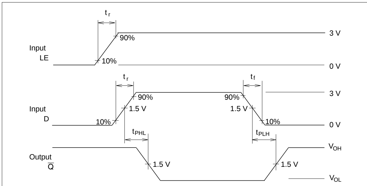
Waveforms-2
