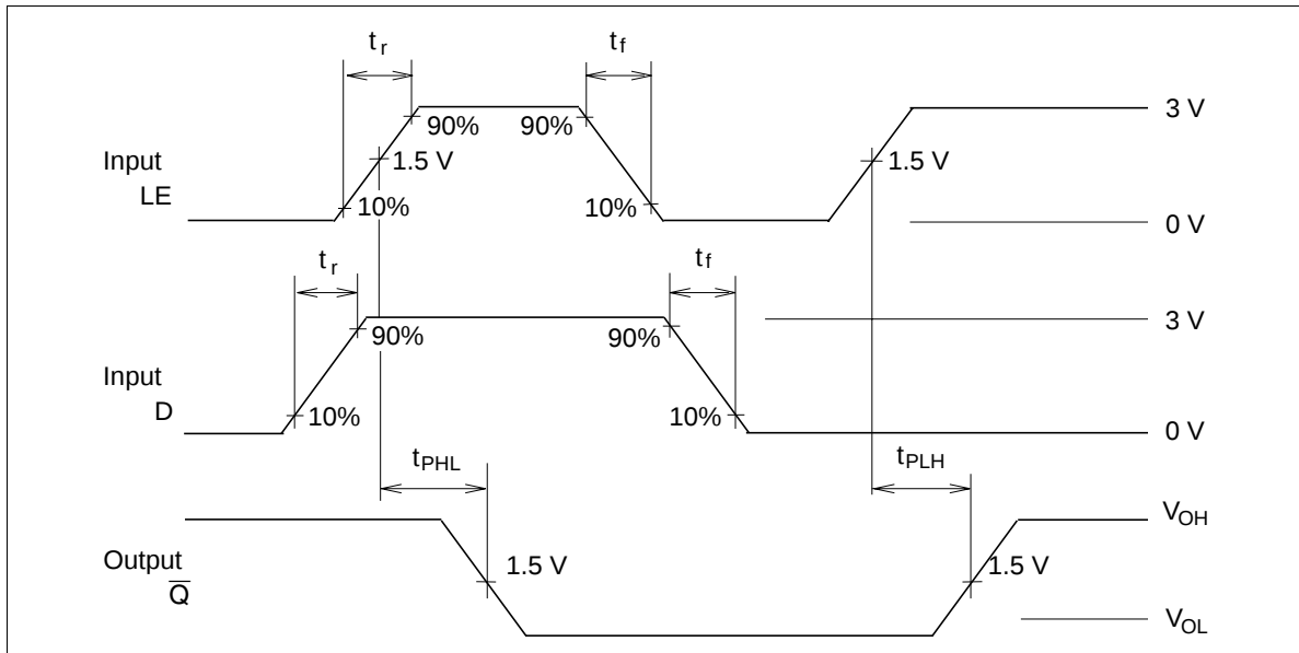
Waveforms-2
