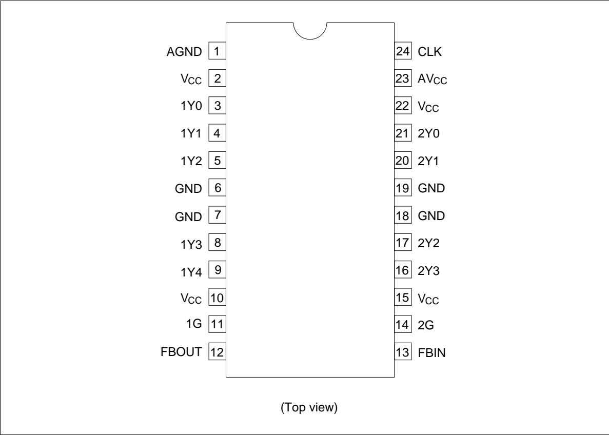
Pin Arrangement
