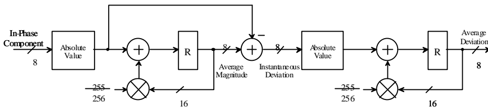
FIGURE 16: NOISE MEASUREMENT CIRCUIT
