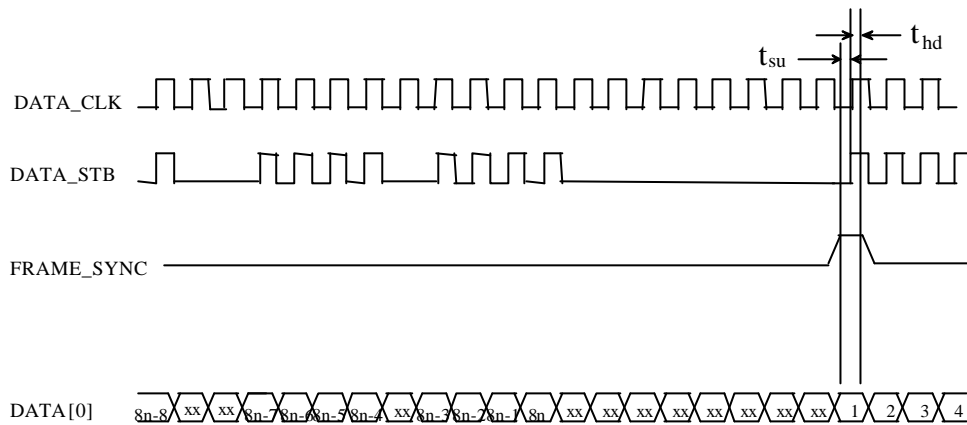
FIGURE 12: OUTPUT TIMING DIAGRAM FOR REGULATED SERIAL MODE1
