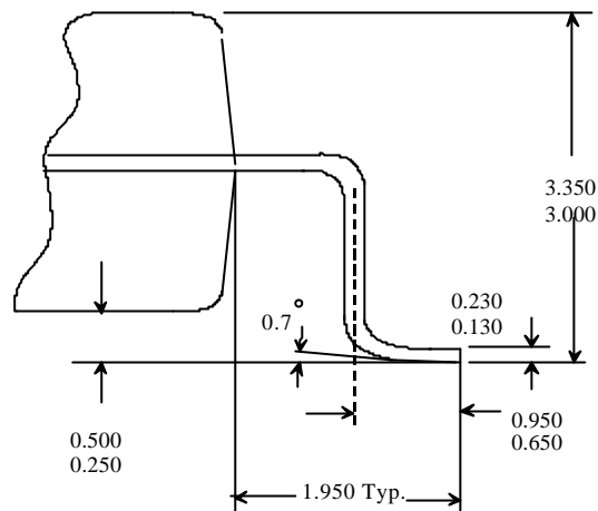
FIGURE 22: MECHANICAL CONFIGURATION
