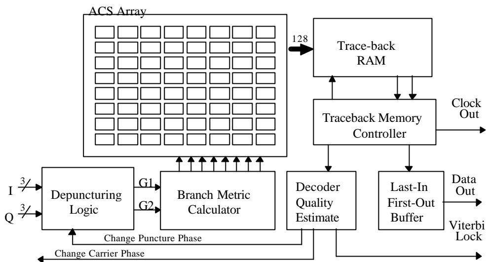
FIGURE 18: VITERBI DECODER
