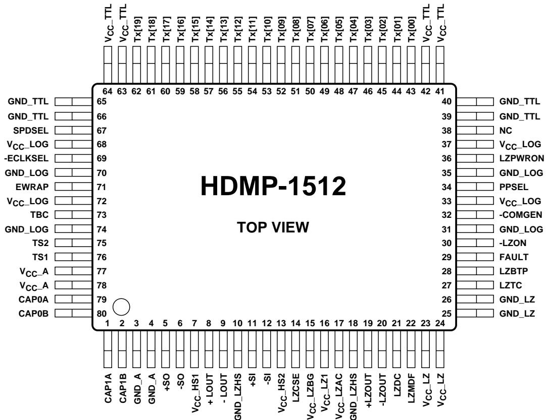
Figure 11. HDMP-1512 (Tx) Package Layout, Top View.
