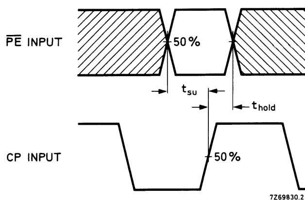
Fig.5 Waveforms showing set-up and hold times for \overline{PE} input. Set-up and hold times are shown as positive values but may be specified as negative values.
