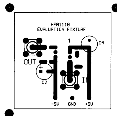
TOP LAYOUT
