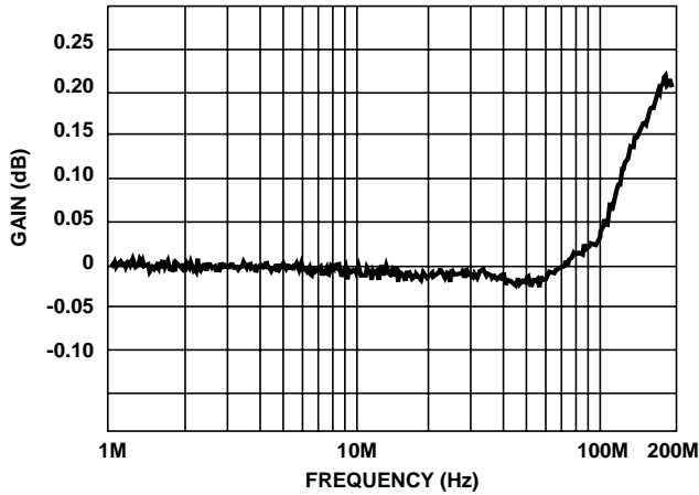
FIGURE 7. GAIN FLATNESS
