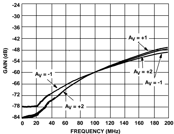
FIGURE 21. LOW FREQUENCY REVERSE ISOLATION ( S_{12} )
