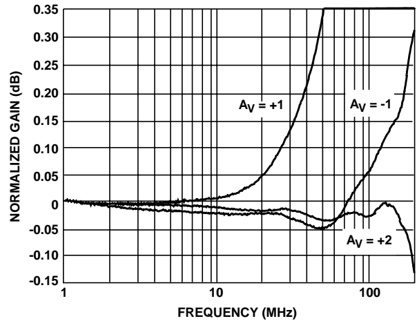
FIGURE 18. GAIN FLATNESS
