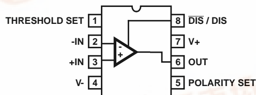
HFA1149 (SOIC) TOP VIEW
