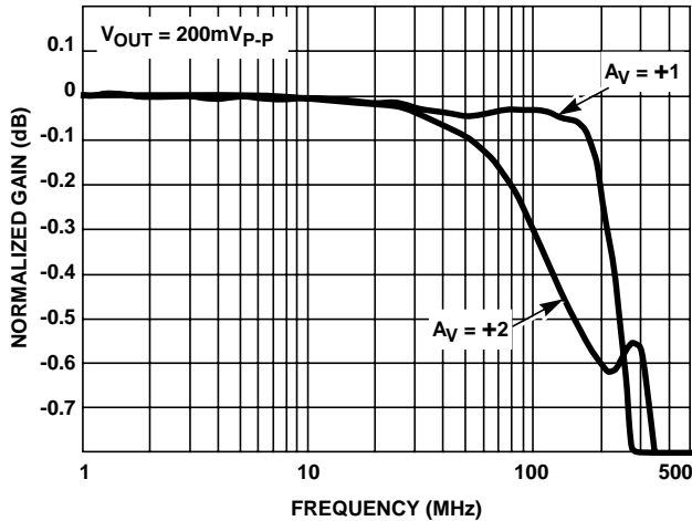
FIGURE 15. GAIN FLATNESS
