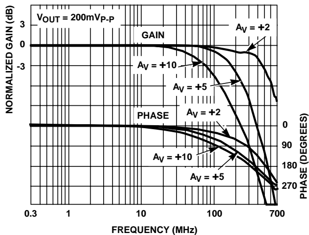
FIGURE 13. FREQUENCY RESPONSE
