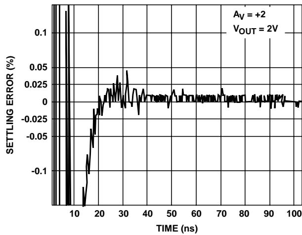
FIGURE 29. SETTLING RESPONSE
