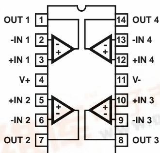
HFA1405 (PDIP, SOIC) TOP VIEW
