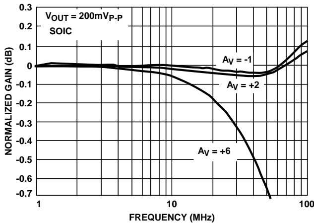
FIGURE 14. GAIN FLATNESS
