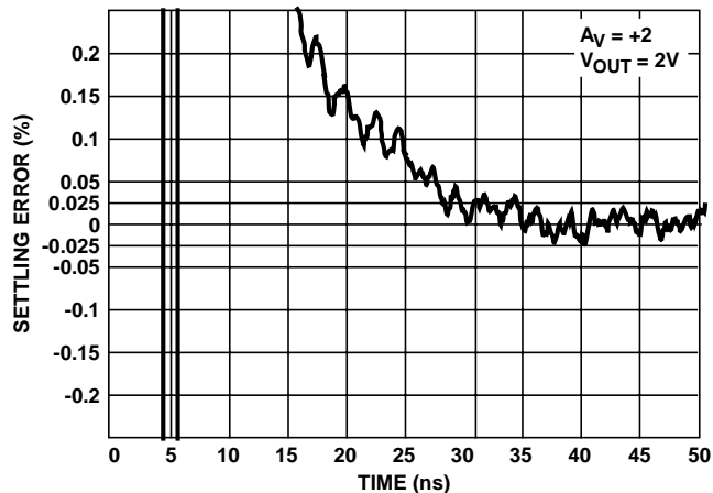
FIGURE 35. SETTLING RESPONSE
