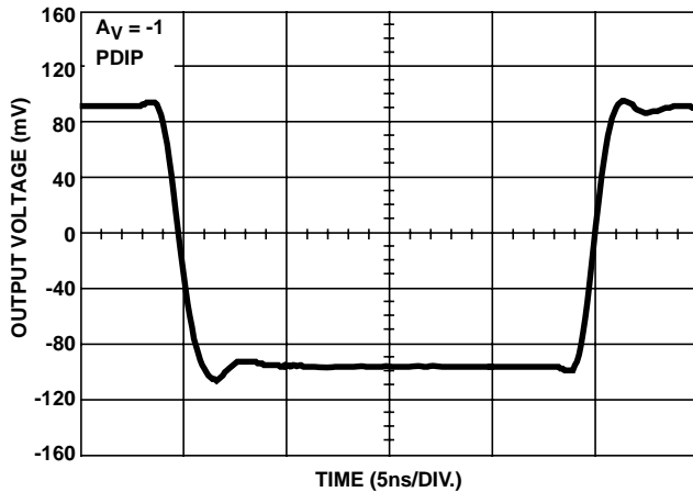
FIGURE 18. SMALL SIGNAL PULSE RESPONSE
