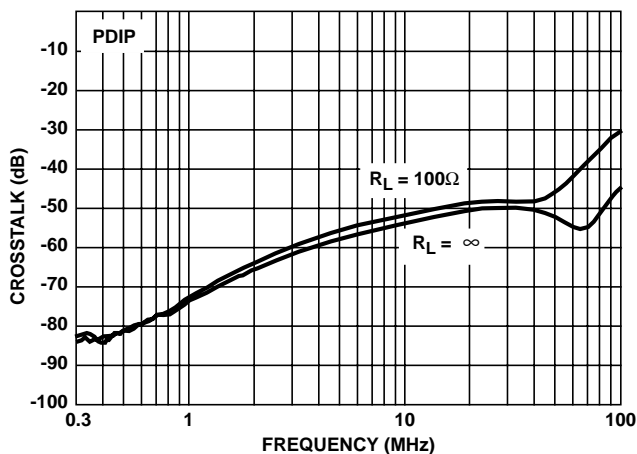
FIGURE 37. ALL HOSTILE CROSSTALK
