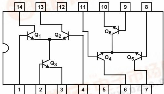
HFA3102 (SOIC) TOP VIEW
