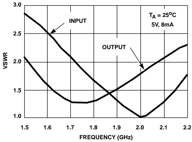
FIGURE 3. VSWR vs FREQUENCY
