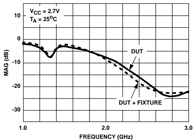
FIGURE 15. LNA S_{22} LOG MAG OUTPUT RETURN LOSS
