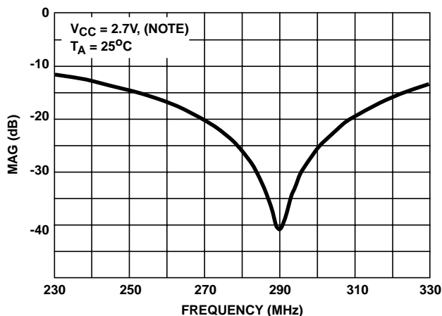
FIGURE 15. LNA S_{22} LOG MAG OUTPUT RETURN LOSS
