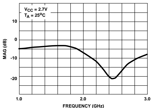
FIGURE 14. LNA S_{12} LOG MAG REVERSE ISOLATION
