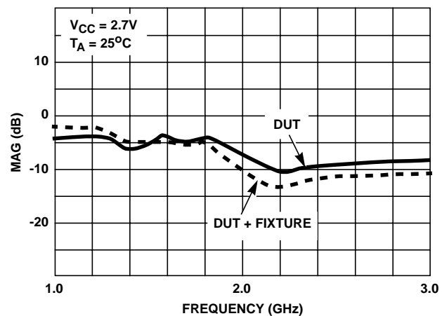
FIGURE 12. LNA S_{11} LOG MAG INPUT RETURN LOSS
