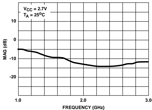
FIGURE 19. RECEIVE MIXER S_{11} LOG MAG RF INPUT RETURN LOSS
