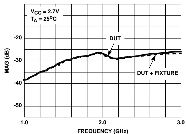
FIGURE 10. PRE-AMPLIFIER S_{12} LOG MAG REVERSE ISOLATION
