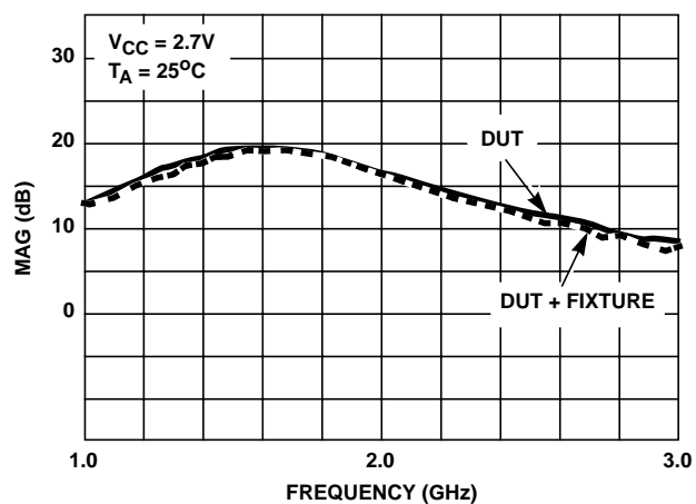
FIGURE 9. PRE-AMPLIFIER S_{21} LOG MAG FORWARD GAIN
