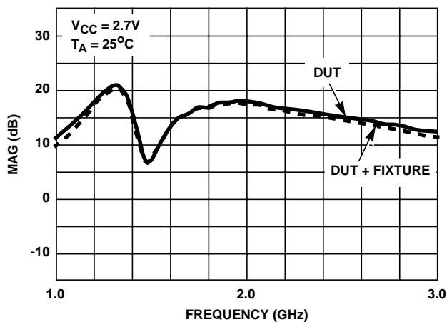
FIGURE 13. LNA S_{21} LOG MAG FORWARD GAIN
