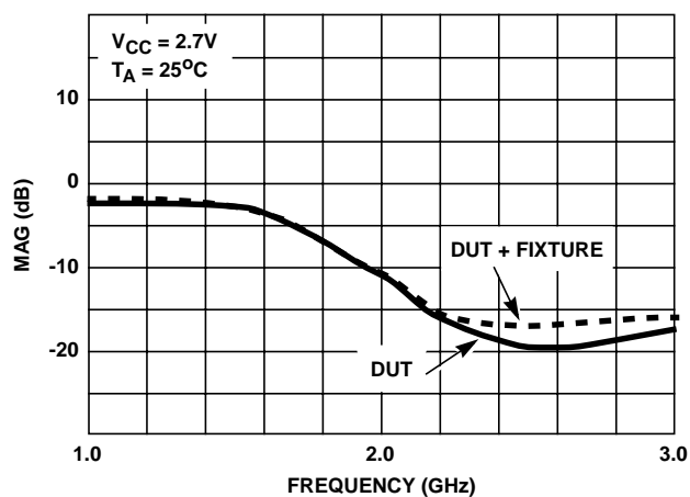
FIGURE 8. PRE-AMPLIFIER S_{11} LOG MAG INPUT RETURN LOSS
