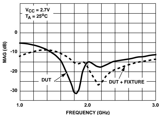
FIGURE 11. PRE-AMPLIFIER S_{22} LOG MAG OUTPUT RETURN LOSS
