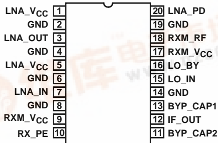
HFA3661 (SSOP) TOP VIEW
