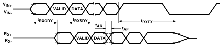
Figure 7. Receive Timing.
