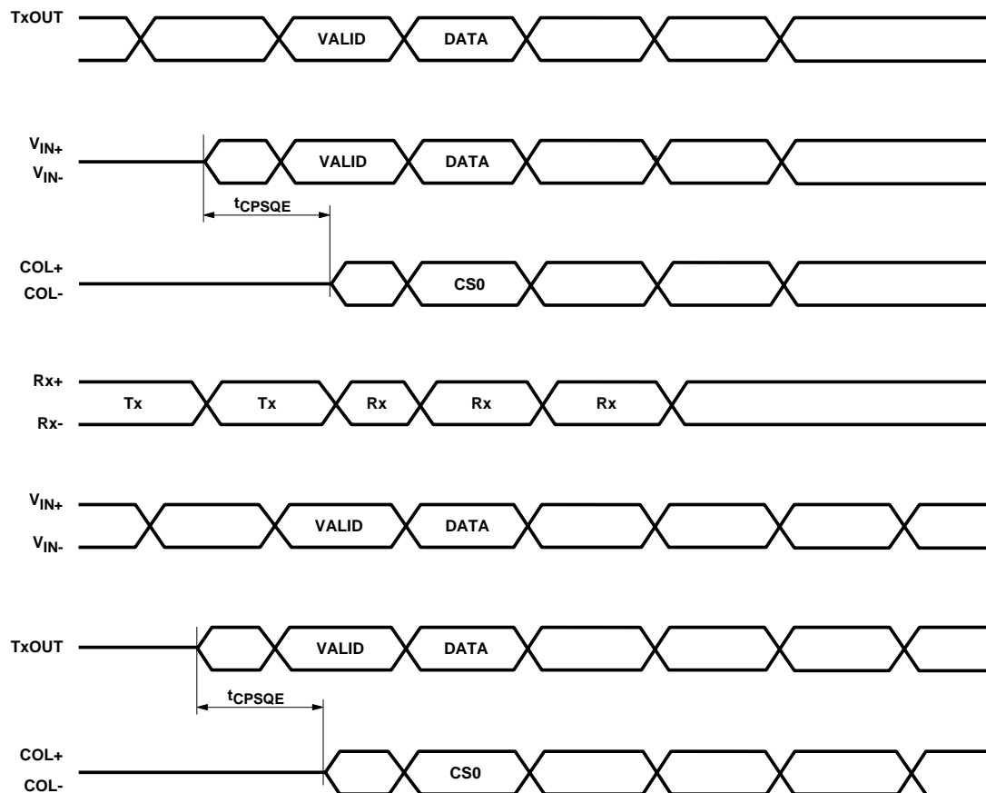
Figure 7. Receive Timing.
