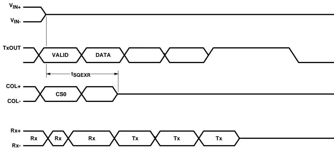
Figure 9. Collision Timing.
