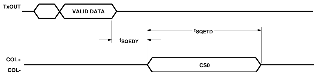
Figure 11. SQE Timing
