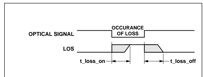
t-loss-on & t-loss-off
