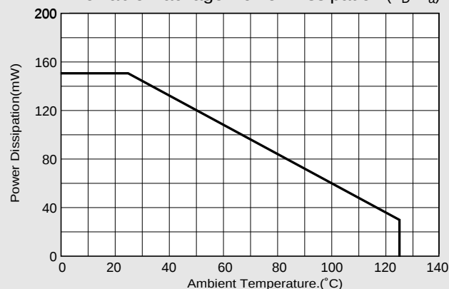
Allowable Package Power Dissipation ( P_{D-T_a} )
