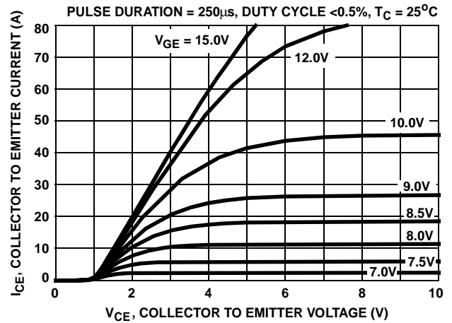
FIGURE 2. SATURATION CHARACTERISTICS
