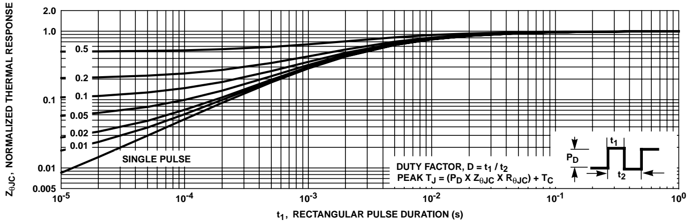
FIGURE 17. NORMALIZED TRANSIENT THERMAL RESPONSE, JUNCTION TO CASE
