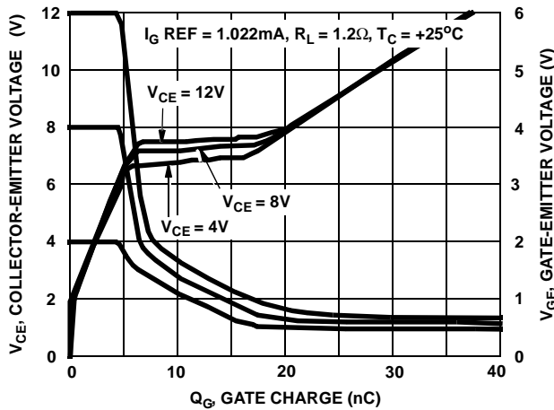
FIGURE 13. GATE CHARGE
