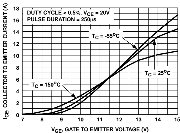
FIGURE 13. TRANSFER CHARACTERISTIC
