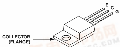
JEDEC TO-220AB (ALTERNATE VERSION)
