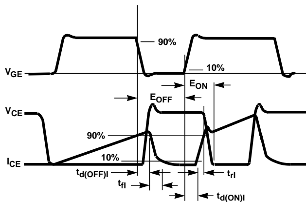
FIGURE 21. SWITCHING TEST WAVEFORMS
