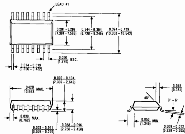
16 Lead Small Outline, Wide (W16) \theta_{JA} = 105^{\circ}\text{C/W} \theta_{JC} = 60^{\circ}\text{C/W}
