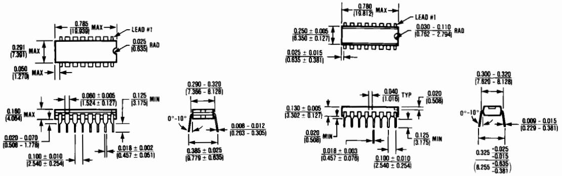
16 Lead CERDIP (HI1) \theta_{JA} = 100^{\circ}\text{C/W} \theta_{JC} = 50^{\circ}\text{C/W}
