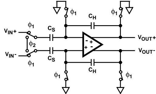
FIGURE 21. ANALOG INPUT SAMPLE-AND-HOLD
