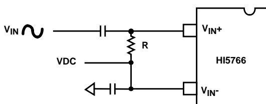
FIGURE 27. AC COUPLED SINGLE ENDED INPUT
