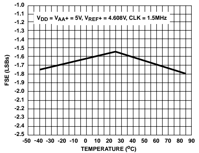
FIGURE 9. FULL SCALE ERROR vs TEMPERATURE
