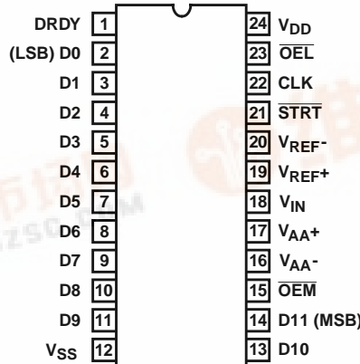
HI5810 (PDIP, CERDIP, SOIC) TOP VIEW
