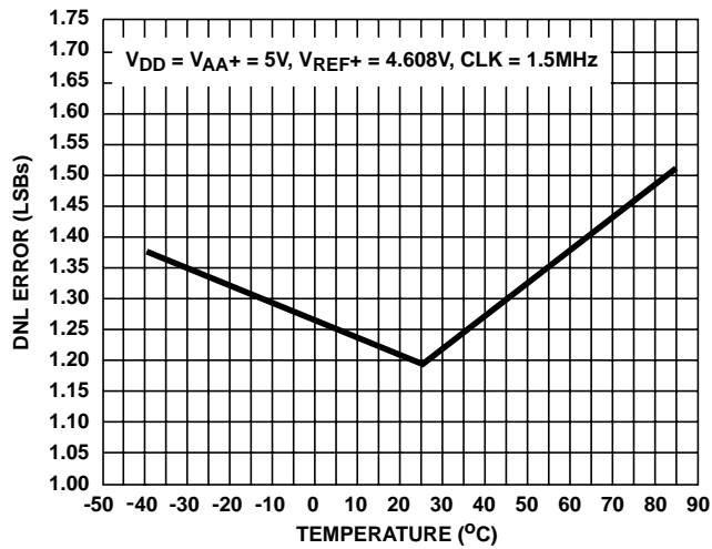
FIGURE 8. DNL vs TEMPERATURE
