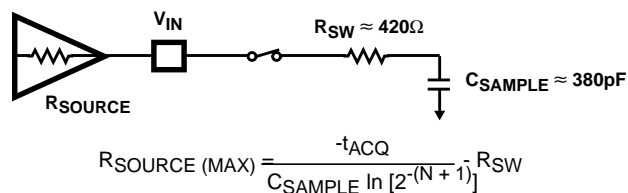
FIGURE 12. ANALOG INPUT MODEL IN TRACK MODE
