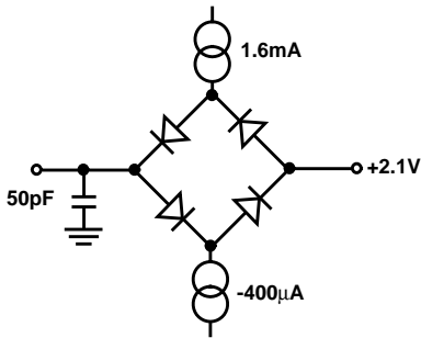
FIGURE 4. GENERAL TIMING LOAD CIRCUIT
