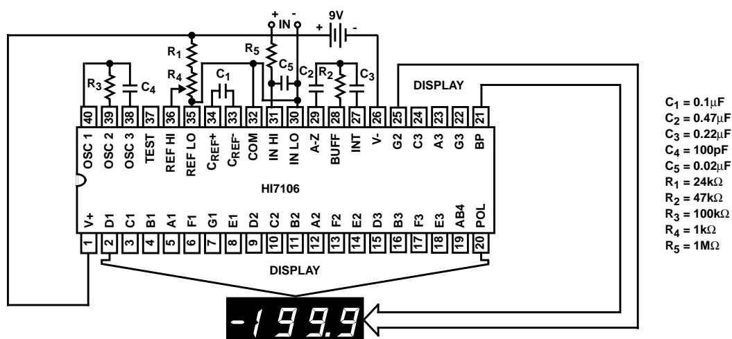
FIGURE 1. HI7106 TEST CIRCUIT AND TYPICAL APPLICATION WITH LCD DISPLAY COMPONENTS SELECTED FOR 200mV FULL SCALE
