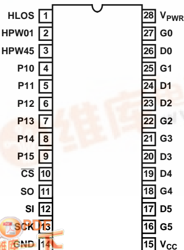
HIP0063 SOIC TOP VIEW
