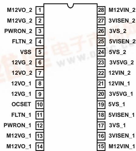
HIP1011D (SSOP) TOP VIEW
